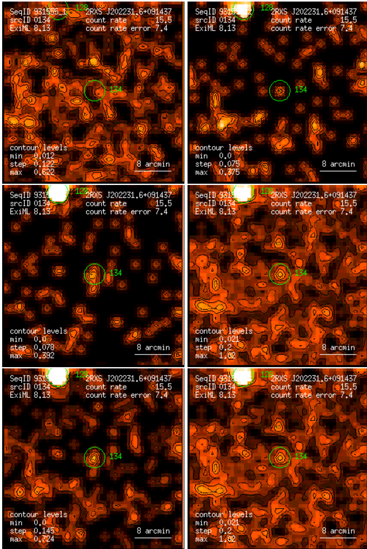
Figure 134: RASS 931555: detection 0134: band rate images, Gaussian filter: (1) PSPC channels 11 – 41, (2) 52 – 90, (3) 91 – 201, (4) 11 – 235, (5) 52 – 201, (6) 11 – 201. Broad band rates in counts/ks. Band rate contour levels in counts/ks/arcmin 2 .
