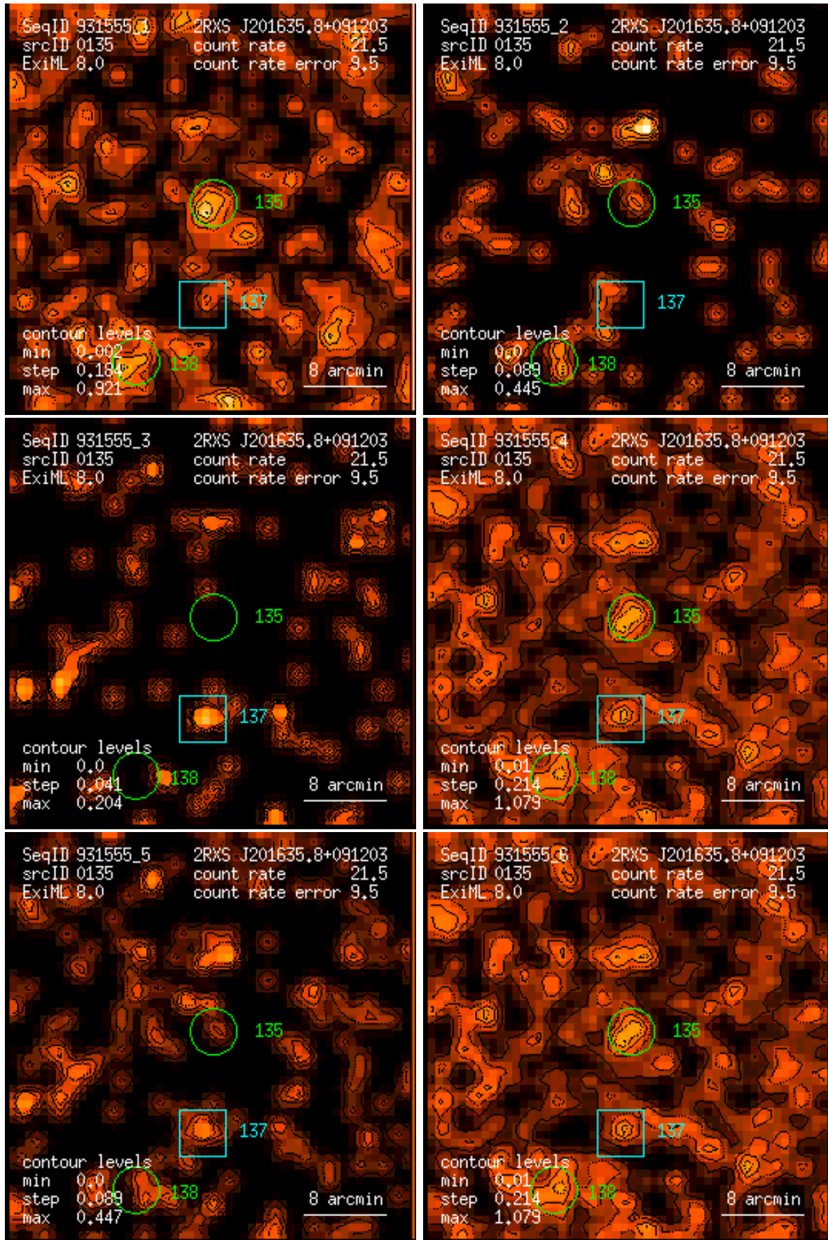
Figure 135: RASS 931555: detection 0135: band rate images, Gaussian filter: (1) PSPC channels 11 – 41, (2) 52 – 90, (3) 91 – 201, (4) 11 – 235, (5) 52 – 201, (6) 11 – 201. Broad band rates in counts/ks. Band rate contour levels in counts/ks/arcmin 2 .
