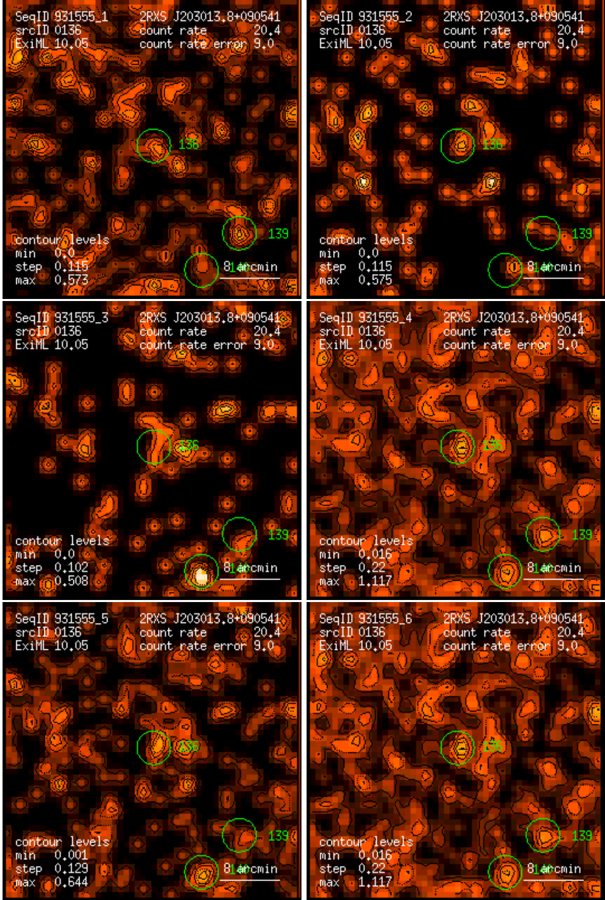
Figure 136: RASS 931555: detection 0136: band rate images, Gaussian filter: (1) PSPC channels 11 – 41, (2) 52 – 90, (3) 91 – 201, (4) 11 – 235, (5) 52 – 201, (6) 11 – 201. Broad band rates in counts/ks. Band rate contour levels in counts/ks/arcmin 2 .
