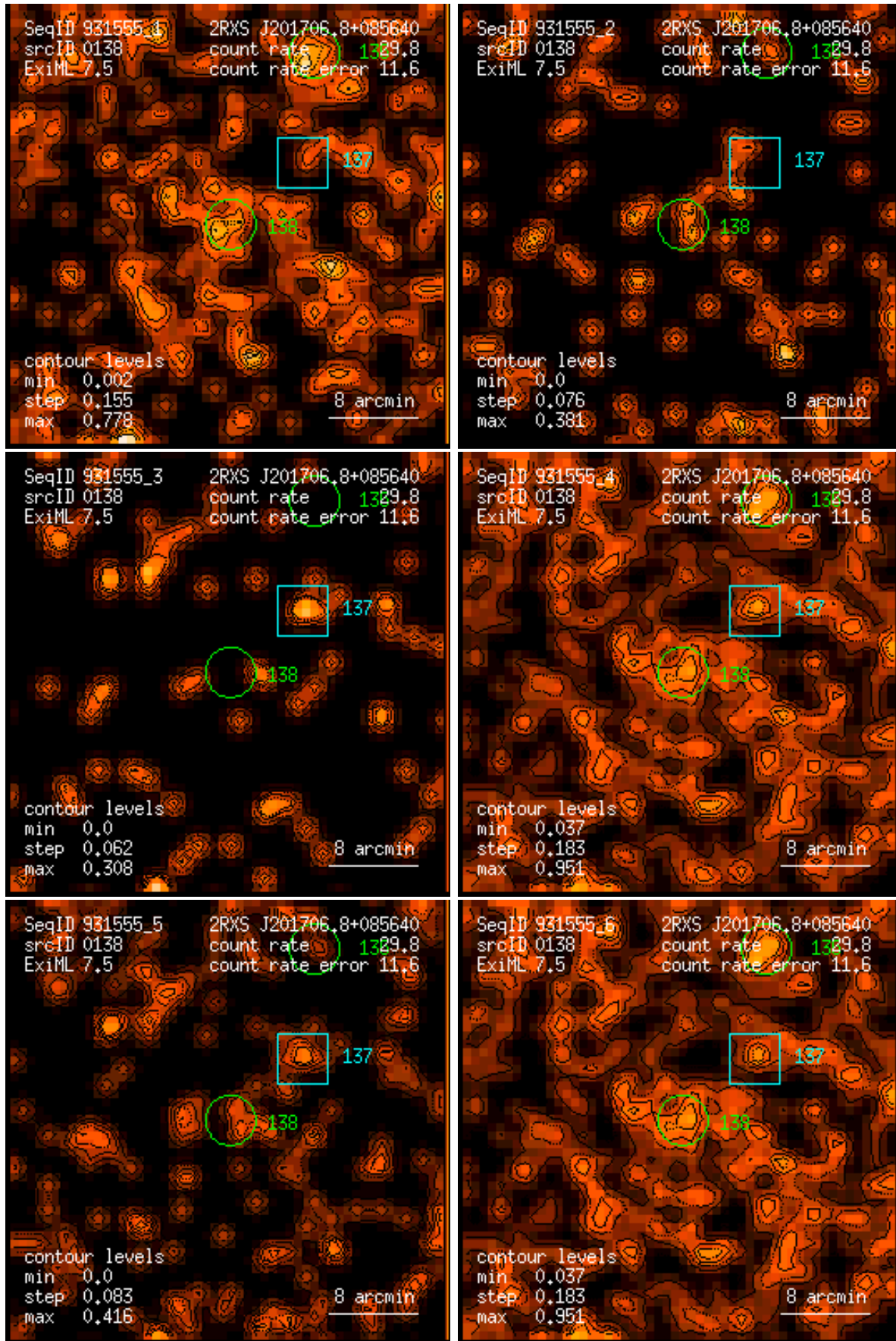
Figure 138: RASS 931555: detection 0138: band rate images, Gaussian filter: (1) PSPC channels 11 – 41, (2) 52 – 90, (3) 91 – 201, (4) 11 – 235, (5) 52 – 201, (6) 11 – 201. Broad band rates in counts/ks. Band rate contour levels in counts/ks/arcmin 2 .
