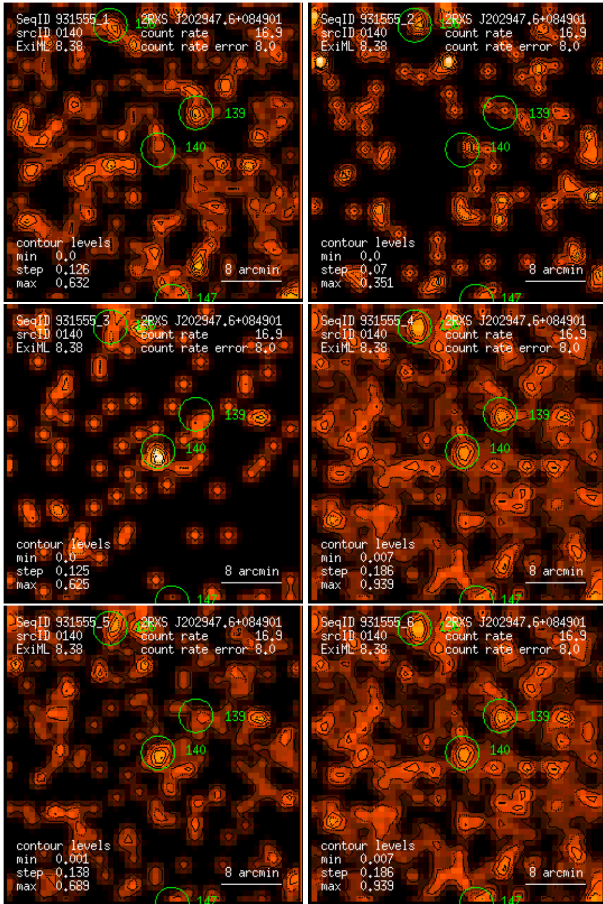
Figure 140: RASS 931555: detection 0140: band rate images, Gaussian filter: (1) PSPC channels 11 – 41, (2) 52 – 90, (3) 91 – 201, (4) 11 – 235, (5) 52 – 201, (6) 11 – 201. Broad band rates in counts/ks. Band rate contour levels in counts/ks/arcmin 2 .
