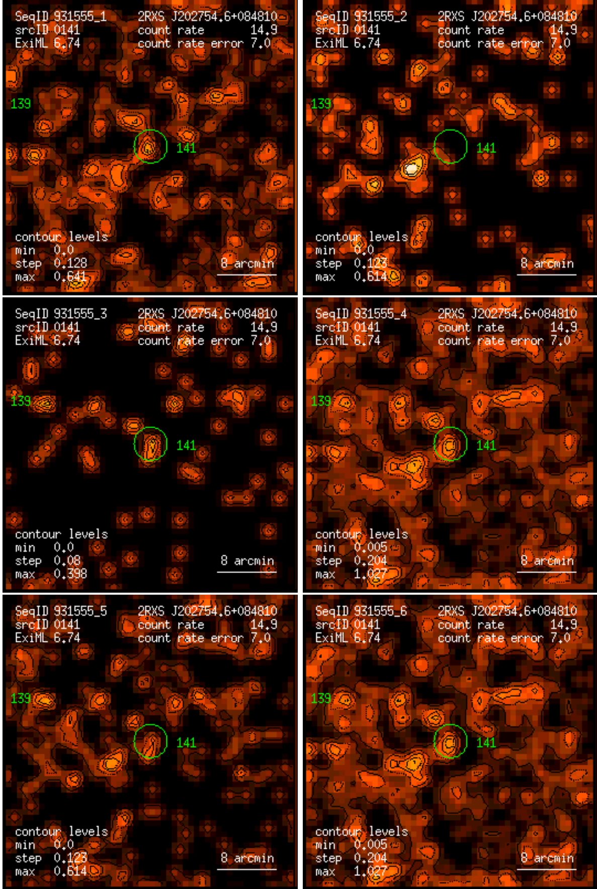
Figure 141: RASS 931555: detection 0141: band rate images, Gaussian filter: (1) PSPC channels 11 – 41, (2) 52 – 90, (3) 91 – 201, (4) 11 – 235, (5) 52 – 201, (6) 11 – 201. Broad band rates in counts/ks. Band rate contour levels in counts/ks/arcmin 2 .
