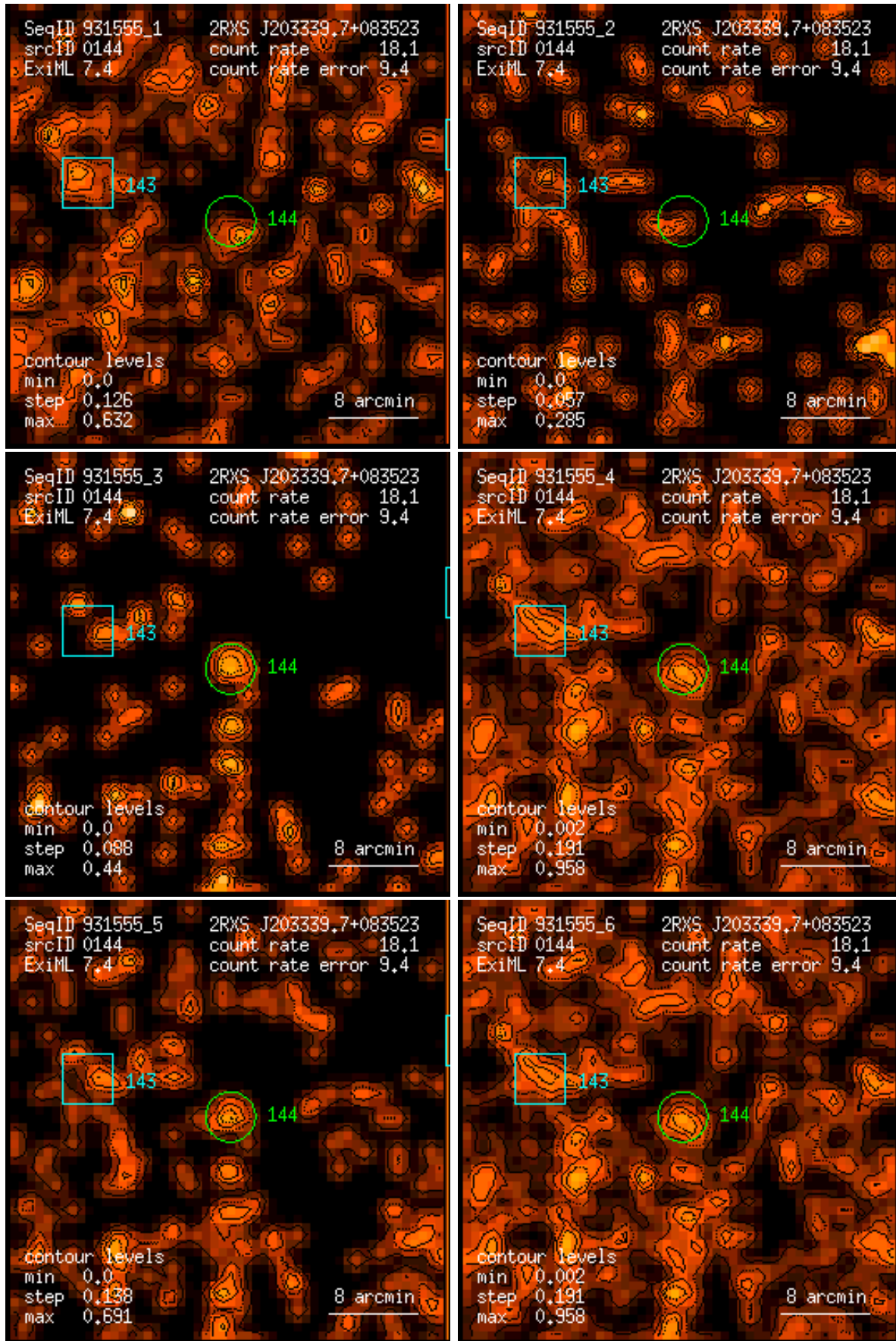
Figure 144: RASS 931555: detection 0144: band rate images, Gaussian filter: (1) PSPC channels 11 – 41, (2) 52 – 90, (3) 91 – 201, (4) 11 – 235, (5) 52 – 201, (6) 11 – 201. Broad band rates in counts/ks. Band rate contour levels in counts/ks/arcmin 2 .
