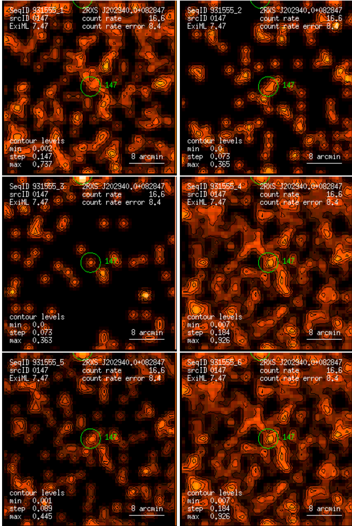
Figure 147: RASS 931555: detection 0147: band rate images, Gaussian filter: (1) PSPC channels 11 – 41, (2) 52 – 90, (3) 91 – 201, (4) 11 – 235, (5) 52 – 201, (6) 11 – 201. Broad band rates in counts/ks. Band rate contour levels in counts/ks/arcmin 2 .
