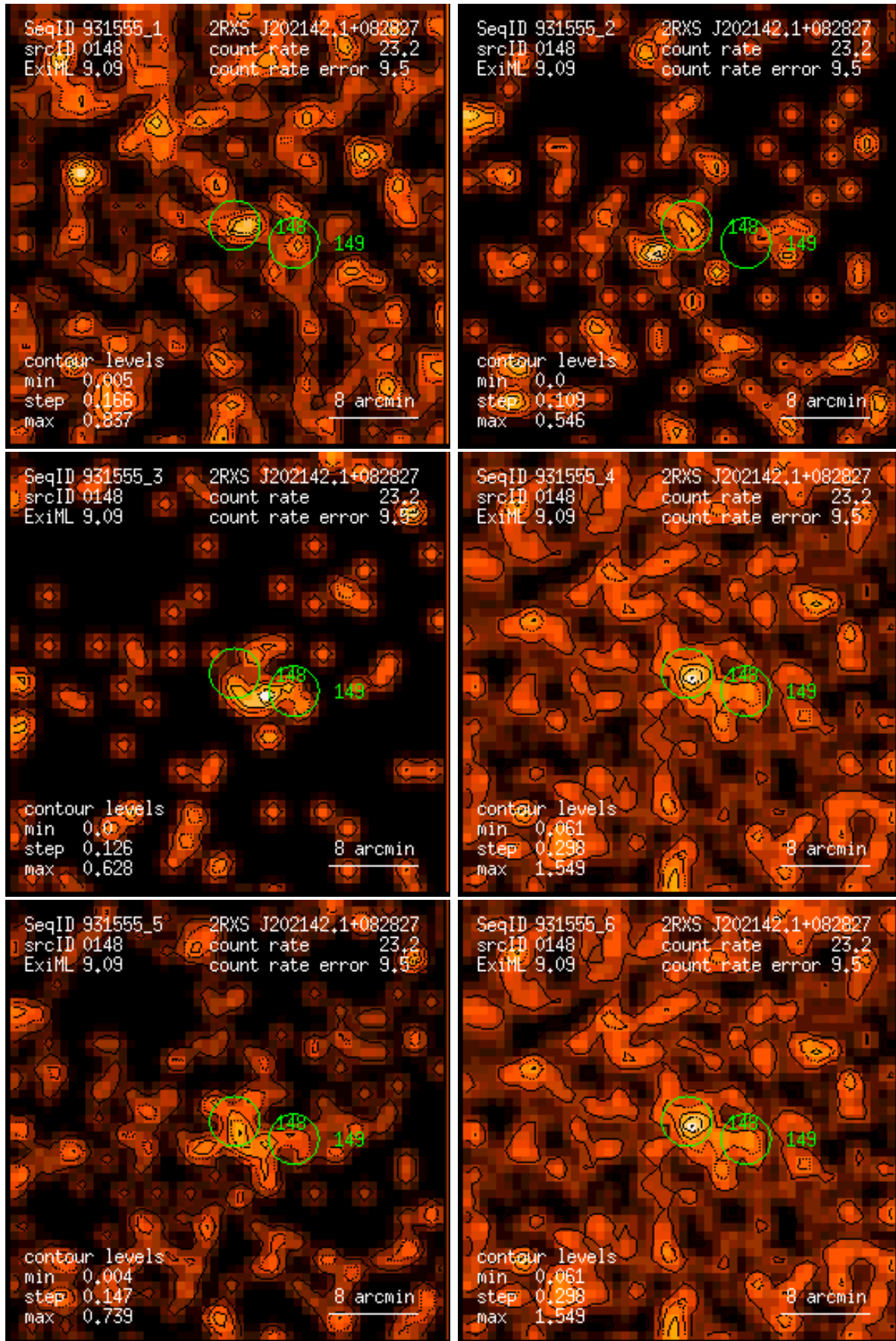
Figure 148: RASS 931555: detection 0148: band rate images, Gaussian filter: (1) PSPC channels 11 – 41, (2) 52 – 90, (3) 91 – 201, (4) 11 – 235, (5) 52 – 201, (6) 11 – 201. Broad band rates in counts/ks. Band rate contour levels in counts/ks/arcmin 2 .
