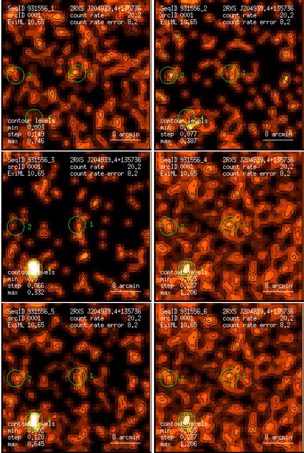
Figure 1: RASS 931556: detection 0001: band rate images, Gaussian filter: (1) PSPC channels 11 – 41, (2) 52 – 90, (3) 91 – 201, (4) 11 – 235, (5) 52 – 201, (6) 11 – 201. Broad band rates in counts/ks. Band rate contour levels in counts/ks/arcmin 2 .
