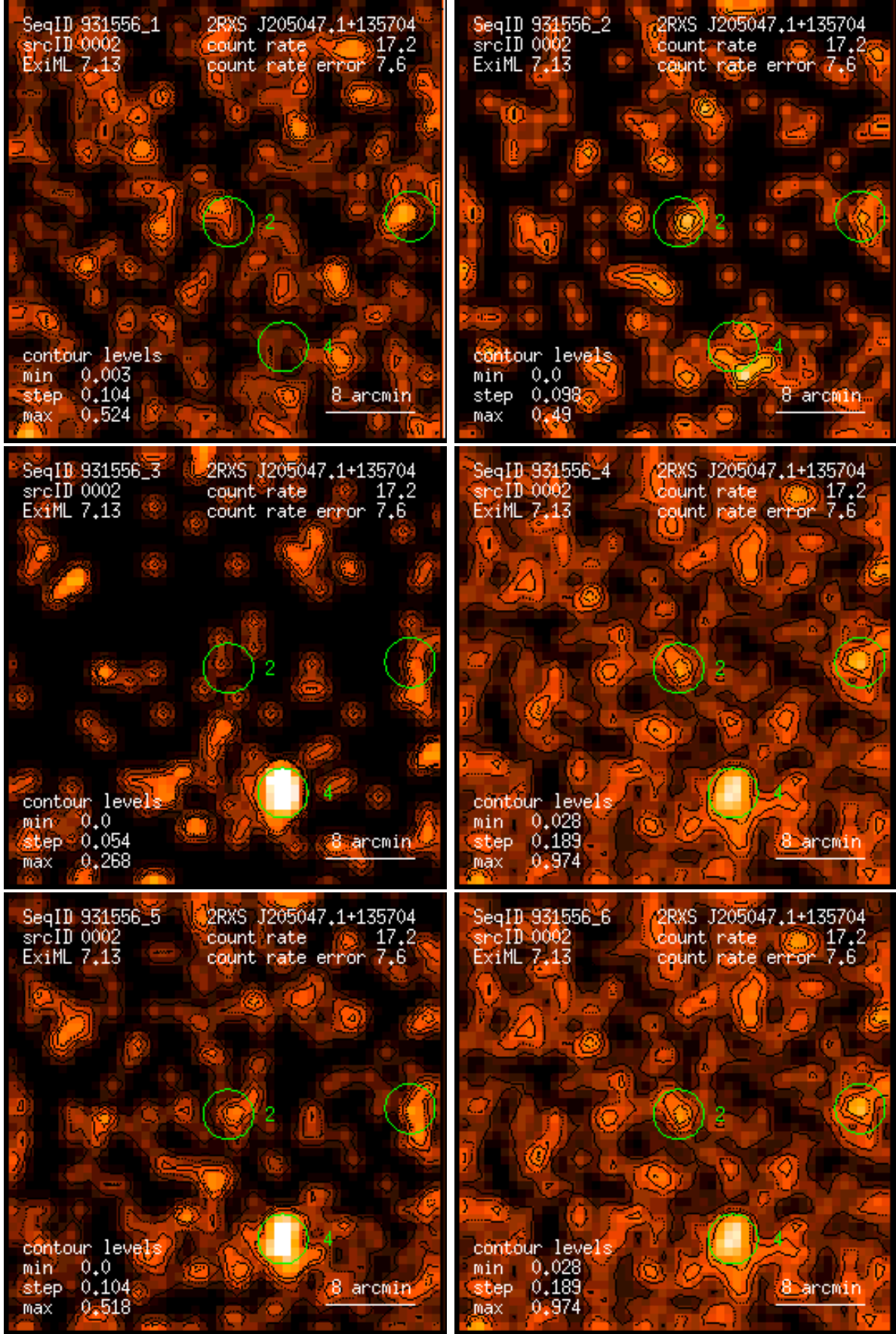
Figure 2: RASS 931556: detection 0002: band rate images, Gaussian filter: (1) PSPC channels 11 – 41, (2) 52 – 90, (3) 91 – 201, (4) 11 – 235, (5) 52 – 201, (6) 11 – 201. Broad band rates in counts/ks. Band rate contour levels in counts/ks/arcmin 2 .
