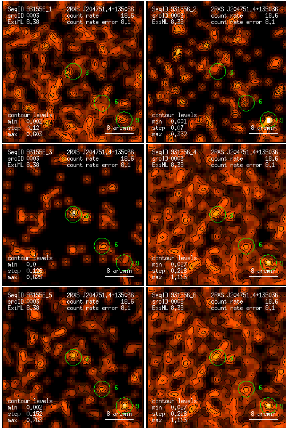
Figure 3: RASS 931556: detection 0003: band rate images, Gaussian filter: (1) PSPC channels 11 – 41, (2) 52 – 90, (3) 91 – 201, (4) 11 – 235, (5) 52 – 201, (6) 11 – 201. Broad band rates in counts/ks. Band rate contour levels in counts/ks/arcmin 2 .
