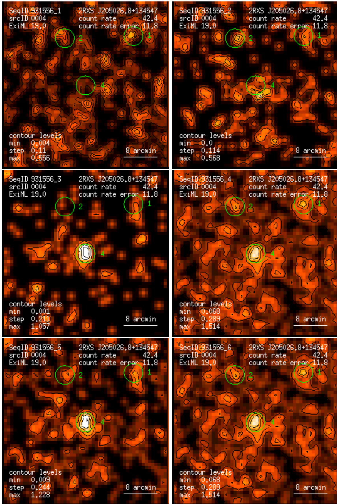
Figure 4: RASS 931556: detection 0004: band rate images, Gaussian filter: (1) PSPC channels 11 – 41, (2) 52 – 90, (3) 91 – 201, (4) 11 – 235, (5) 52 – 201, (6) 11 – 201. Broad band rates in counts/ks. Band rate contour levels in counts/ks/arcmin 2 .
