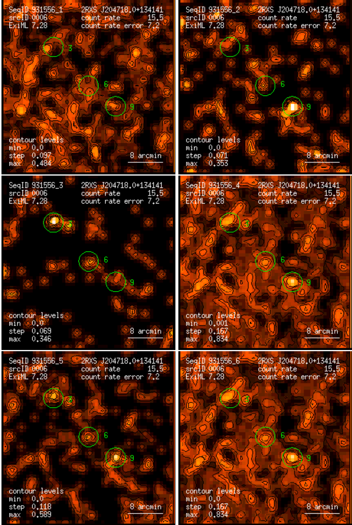
Figure 6: RASS 931556: detection 0006: band rate images, Gaussian filter: (1) PSPC channels 11 – 41, (2) 52 – 90, (3) 91 – 201, (4) 11 – 235, (5) 52 – 201, (6) 11 – 201. Broad band rates in counts/ks. Band rate contour levels in counts/ks/arcmin 2 .
