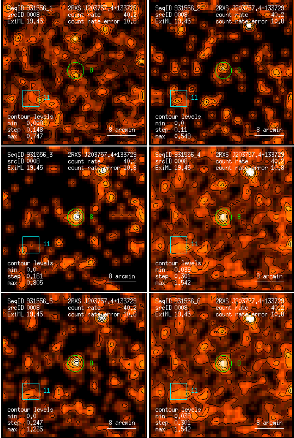
Figure 8: RASS 931556: detection 0008: band rate images, Gaussian filter: (1) PSPC channels 11 – 41, (2) 52 – 90, (3) 91 – 201, (4) 11 – 235, (5) 52 – 201, (6) 11 – 201. Broad band rates in counts/ks. Band rate contour levels in counts/ks/arcmin 2 .
