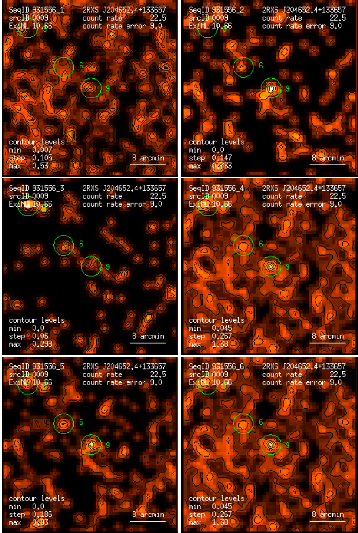
Figure 9: RASS 931556: detection 0009: band rate images, Gaussian filter: (1) PSPC channels 11 – 41, (2) 52 – 90, (3) 91 – 201, (4) 11 – 235, (5) 52 – 201, (6) 11 – 201. Broad band rates in counts/ks. Band rate contour levels in counts/ks/arcmin 2 .
