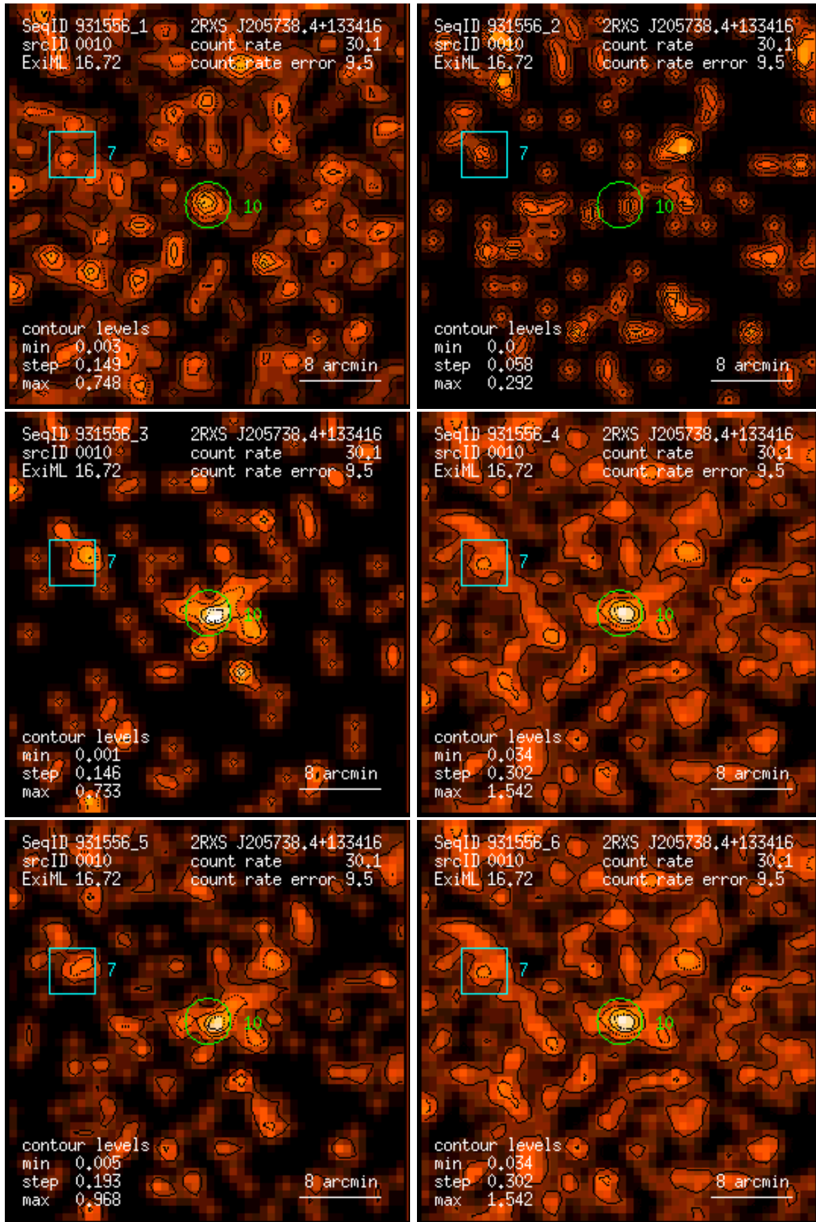
Figure 10: RASS 931556: detection 0010: band rate images, Gaussian filter: (1) PSPC channels 11 – 41, (2) 52 – 90, (3) 91 – 201, (4) 11 – 235, (5) 52 – 201, (6) 11 – 201. Broad band rates in counts/ks. Band rate contour levels in counts/ks/arcmin 2 .
