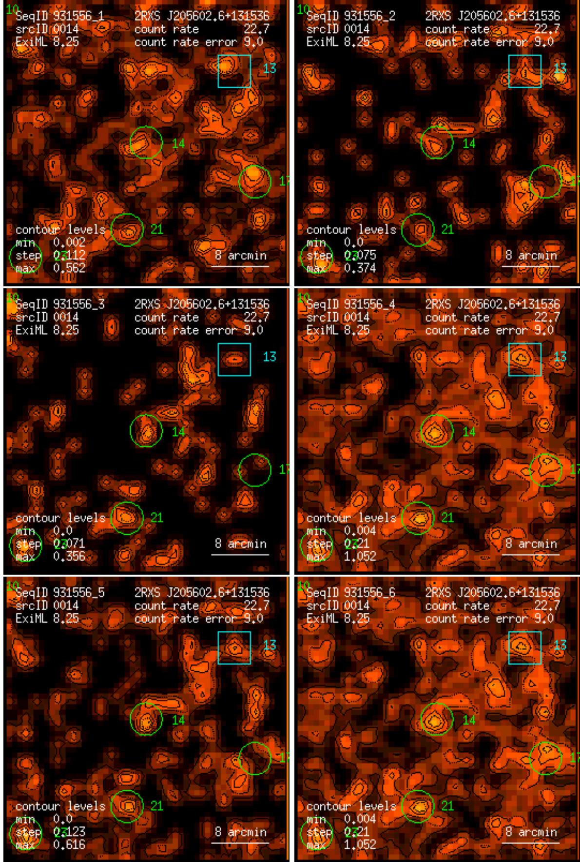
Figure 14: RASS 931556: detection 0014: band rate images, Gaussian filter: (1) PSPC channels 11 – 41, (2) 52 – 90, (3) 91 – 201, (4) 11 – 235, (5) 52 – 201, (6) 11 – 201. Broad band rates in counts/ks. Band rate contour levels in counts/ks/arcmin 2 .
