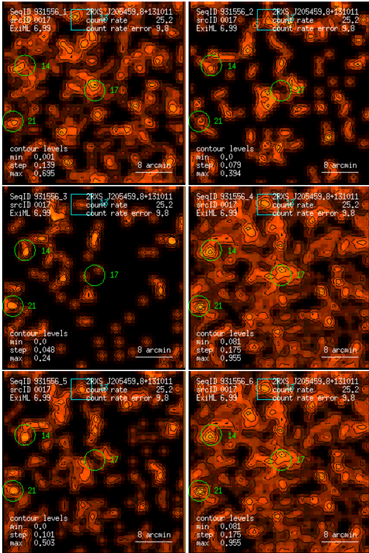
Figure 17: RASS 931556: detection 0017: band rate images, Gaussian filter: (1) PSPC channels 11 – 41, (2) 52 – 90, (3) 91 – 201, (4) 11 – 235, (5) 52 – 201, (6) 11 – 201. Broad band rates in counts/ks. Band rate contour levels in counts/ks/arcmin 2 .
