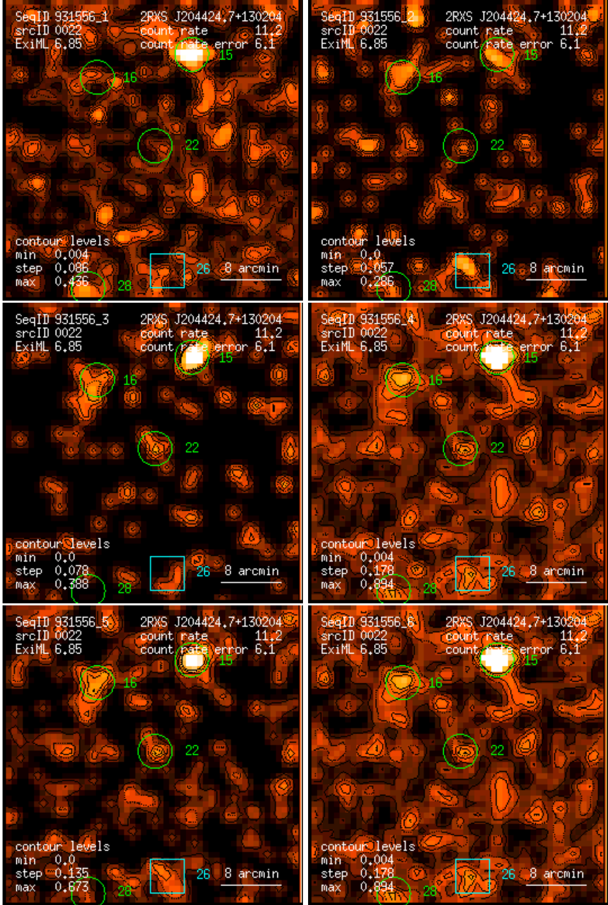
Figure 22: RASS 931556: detection 0022: band rate images, Gaussian filter: (1) PSPC channels 11 – 41, (2) 52 – 90, (3) 91 – 201, (4) 11 – 235, (5) 52 – 201, (6) 11 – 201. Broad band rates in counts/ks. Band rate contour levels in counts/ks/arcmin 2 .
