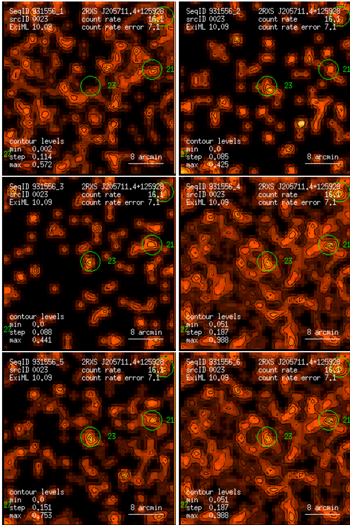
Figure 23: RASS 931556: detection 0023: band rate images, Gaussian filter: (1) PSPC channels 11 – 41, (2) 52 – 90, (3) 91 – 201, (4) 11 – 235, (5) 52 – 201, (6) 11 – 201. Broad band rates in counts/ks. Band rate contour levels in counts/ks/arcmin 2 .
