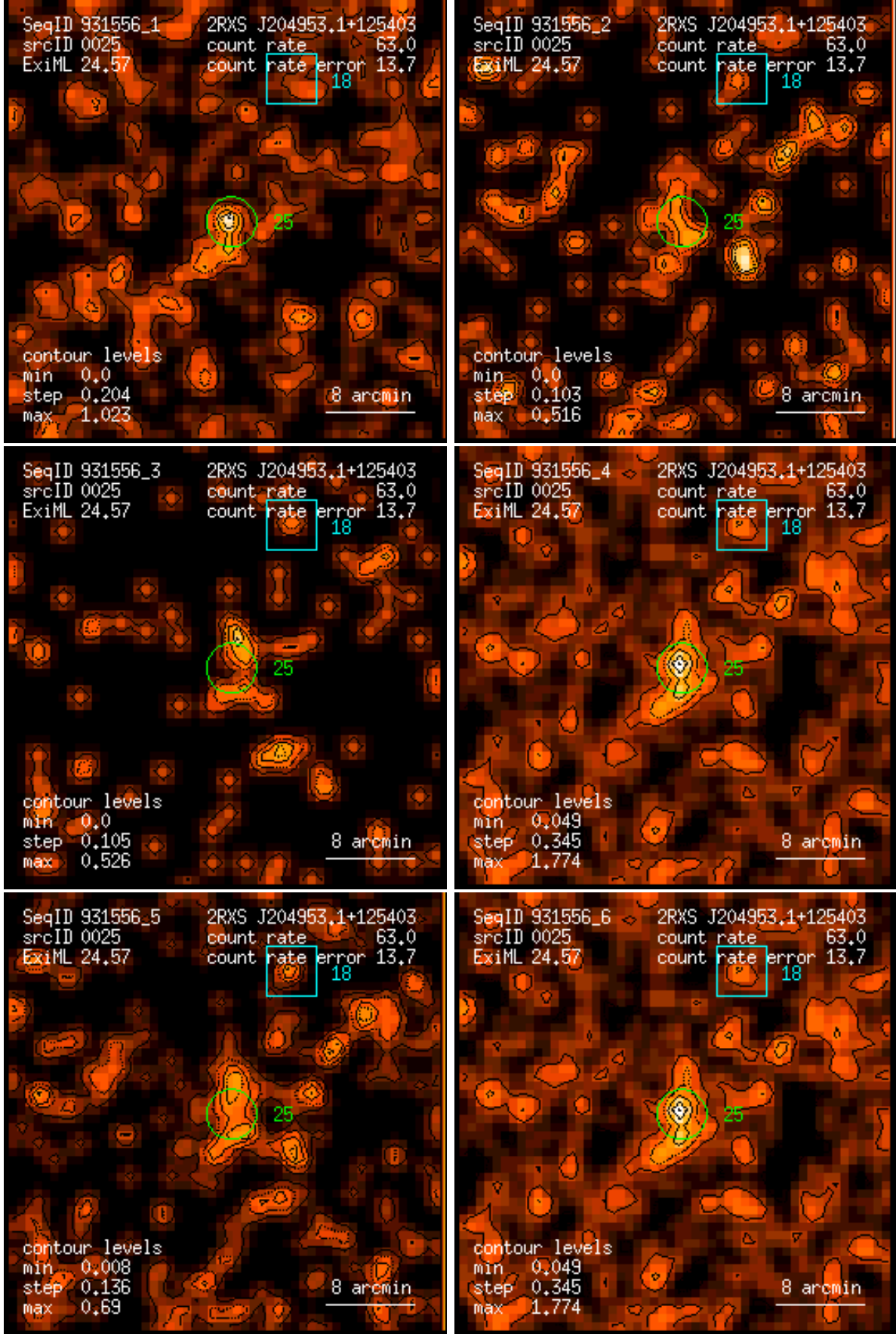
Figure 25: RASS 931556: detection 0025: band rate images, Gaussian filter: (1) PSPC channels 11 – 41, (2) 52 – 90, (3) 91 – 201, (4) 11 – 235, (5) 52 – 201, (6) 11 – 201. Broad band rates in counts/ks. Band rate contour levels in counts/ks/arcmin 2 .
