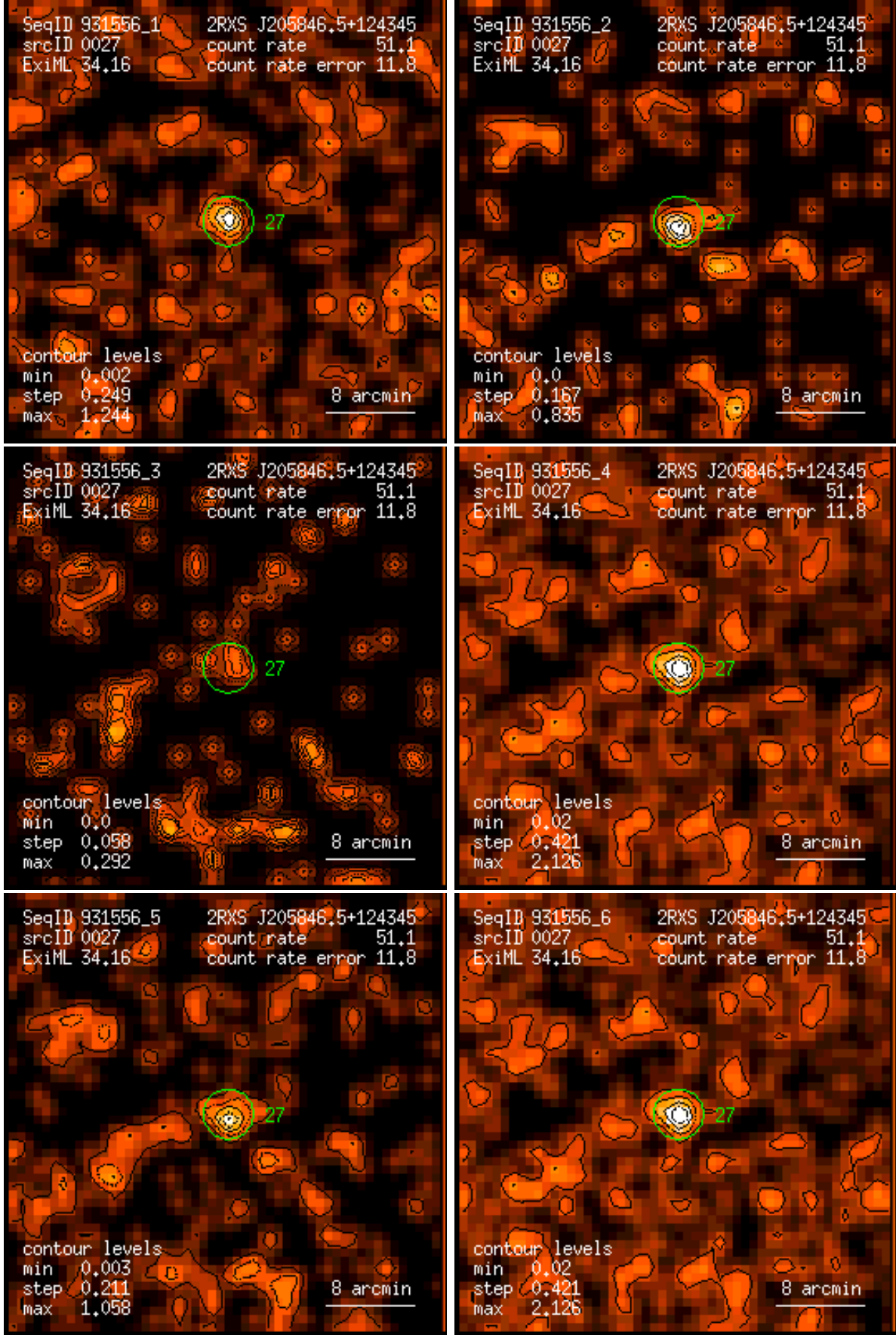
Figure 27: RASS 931556: detection 0027: band rate images, Gaussian filter: (1) PSPC channels 11 – 41, (2) 52 – 90, (3) 91 – 201, (4) 11 – 235, (5) 52 – 201, (6) 11 – 201. Broad band rates in counts/ks. Band rate contour levels in counts/ks/arcmin 2 .
