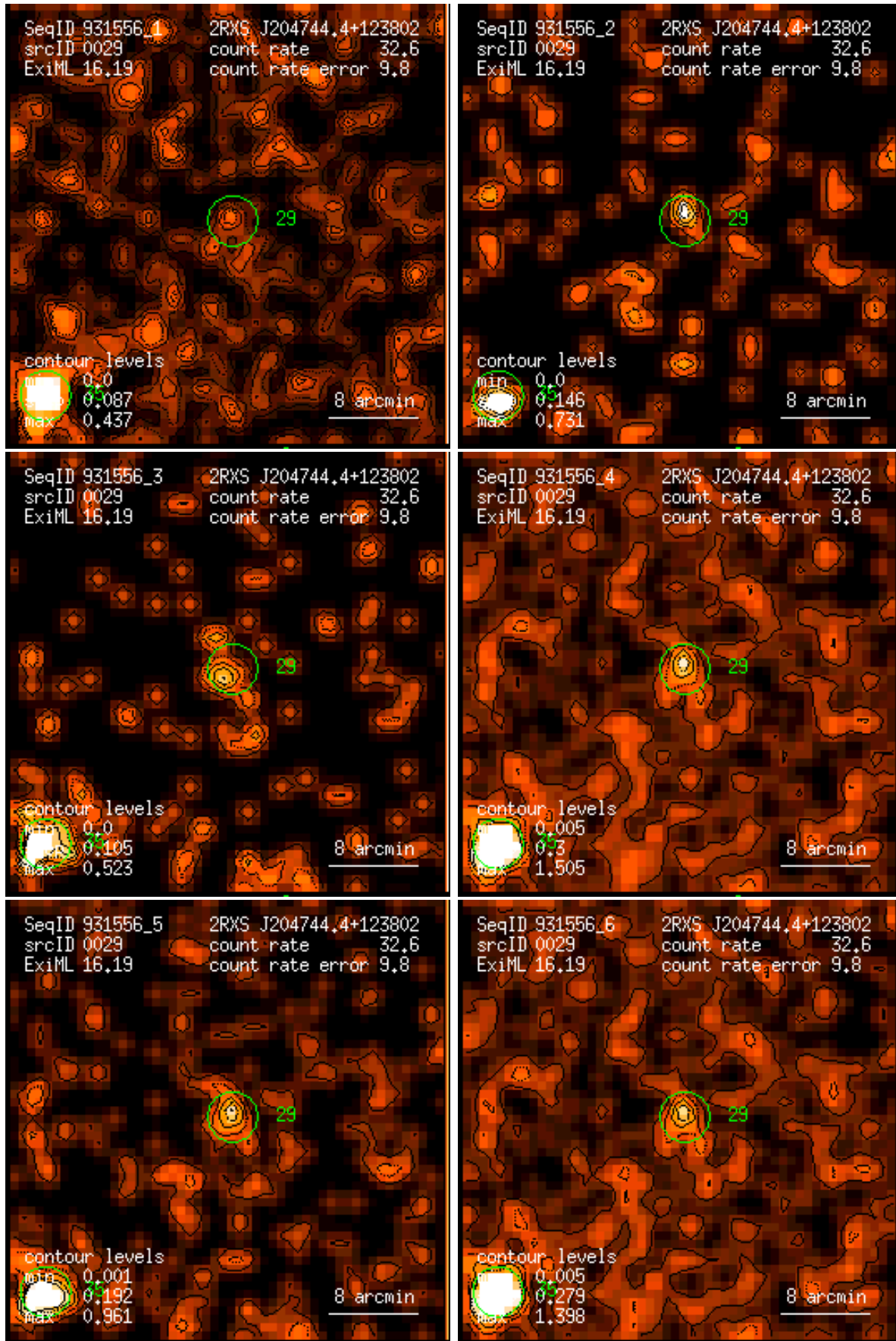
Figure 29: RASS 931556: detection 0029: band rate images, Gaussian filter: (1) PSPC channels 11 – 41, (2) 52 – 90, (3) 91 – 201, (4) 11 – 235, (5) 52 – 201, (6) 11 – 201. Broad band rates in counts/ks. Band rate contour levels in counts/ks/arcmin 2 .
