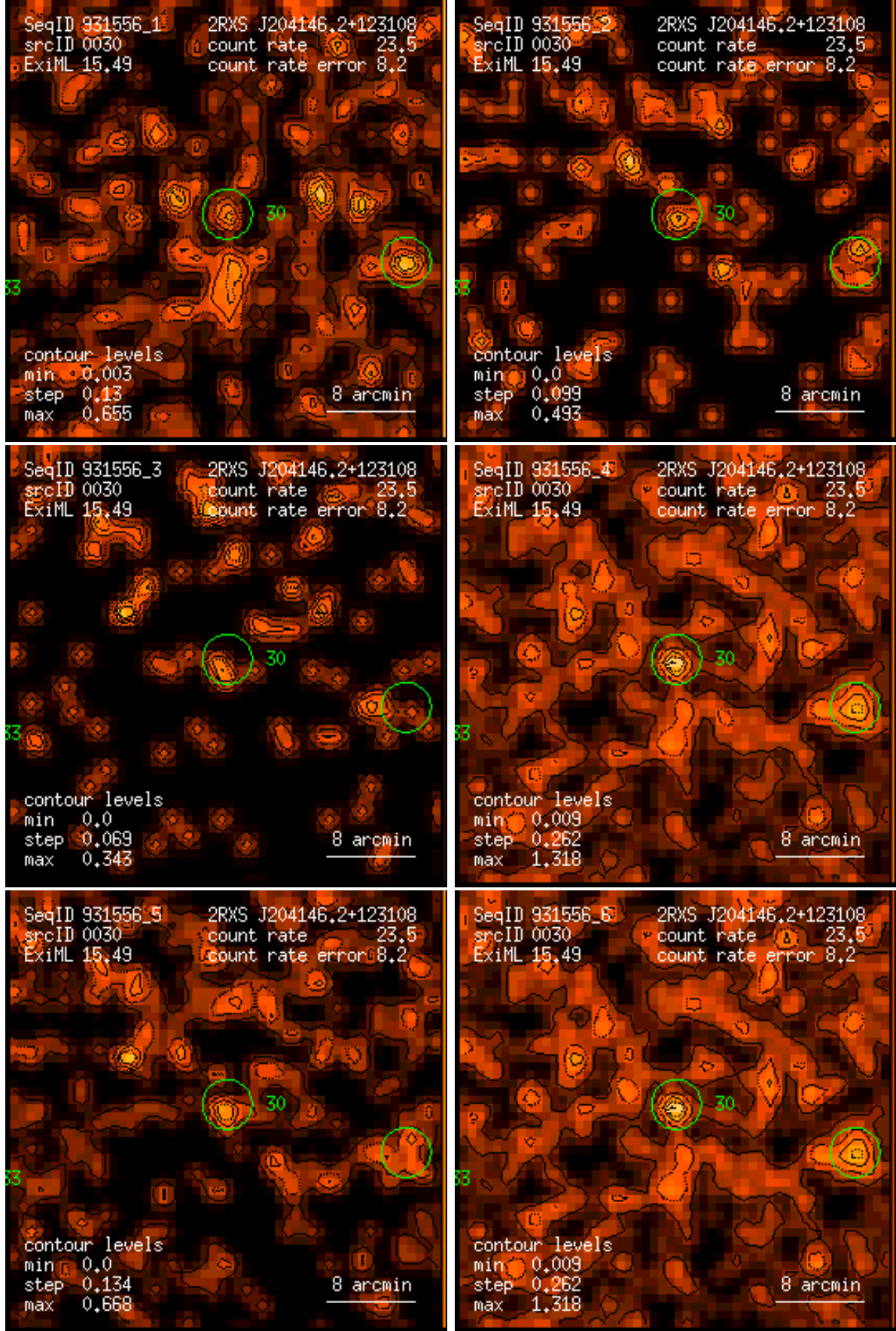
Figure 30: RASS 931556: detection 0030: band rate images, Gaussian filter: (1) PSPC channels 11 – 41, (2) 52 – 90, (3) 91 – 201, (4) 11 – 235, (5) 52 – 201, (6) 11 – 201. Broad band rates in counts/ks. Band rate contour levels in counts/ks/arcmin 2 .
