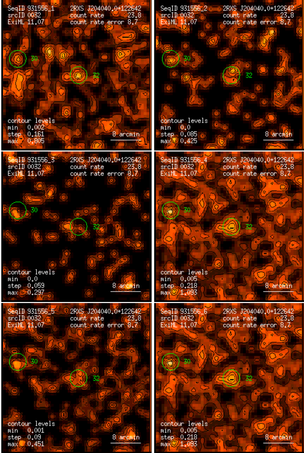
Figure 32: RASS 931556: detection 0032: band rate images, Gaussian filter: (1) PSPC channels 11 – 41, (2) 52 – 90, (3) 91 – 201, (4) 11 – 235, (5) 52 – 201, (6) 11 – 201. Broad band rates in counts/ks. Band rate contour levels in counts/ks/arcmin 2 .
