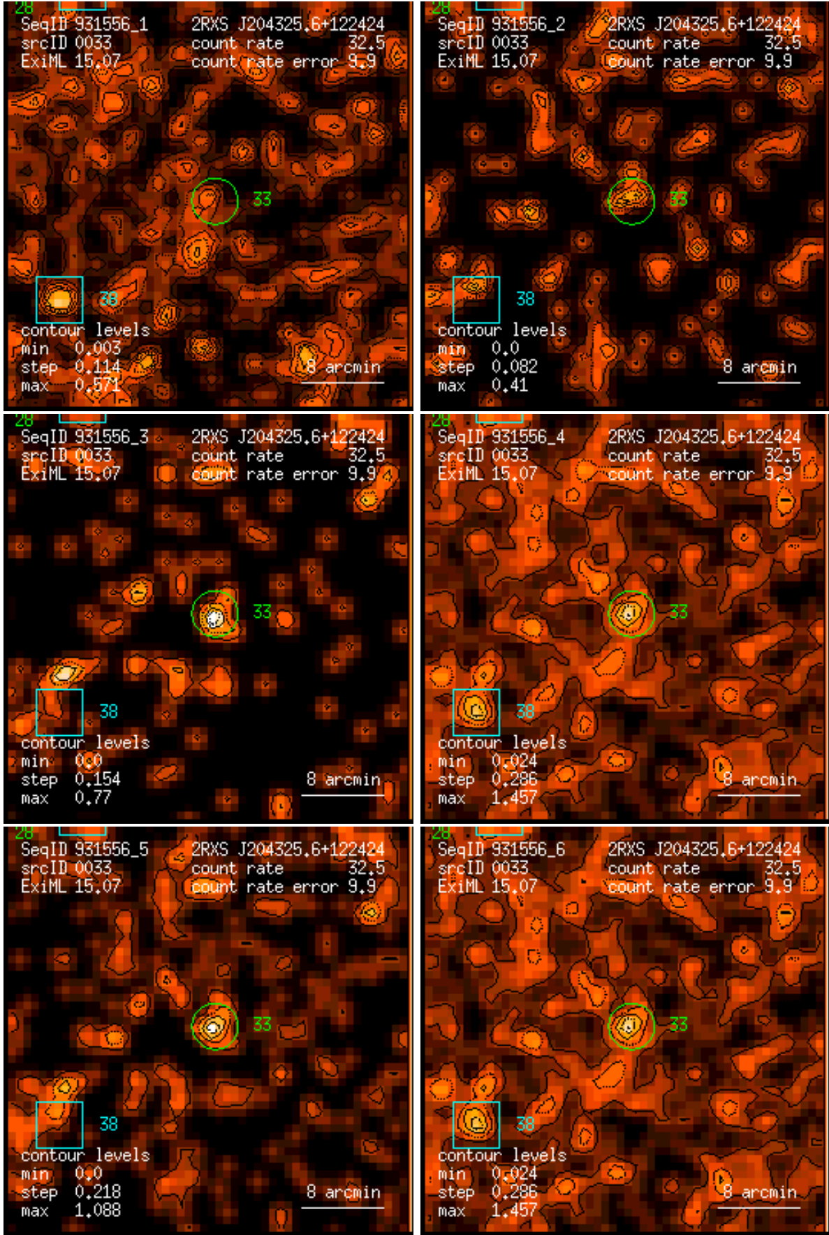
Figure 33: RASS 931556: detection 0033: band rate images, Gaussian filter: (1) PSPC channels 11 – 41, (2) 52 – 90, (3) 91 – 201, (4) 11 – 235, (5) 52 – 201, (6) 11 – 201. Broad band rates in counts/ks. Band rate contour levels in counts/ks/arcmin 2 .
