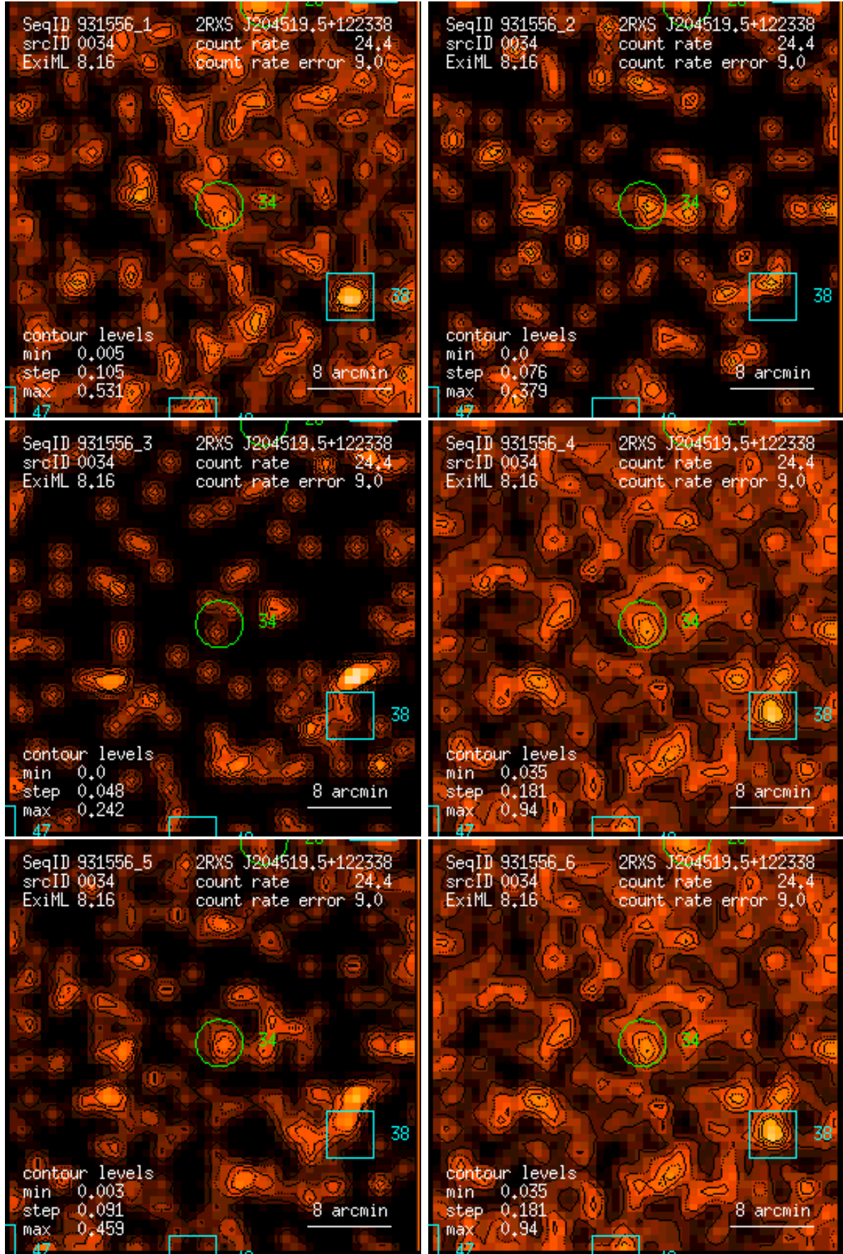
Figure 34: RASS 931556: detection 0034: band rate images, Gaussian filter: (1) PSPC channels 11 – 41, (2) 52 – 90, (3) 91 – 201, (4) 11 – 235, (5) 52 – 201, (6) 11 – 201. Broad band rates in counts/ks. Band rate contour levels in counts/ks/arcmin 2 .
