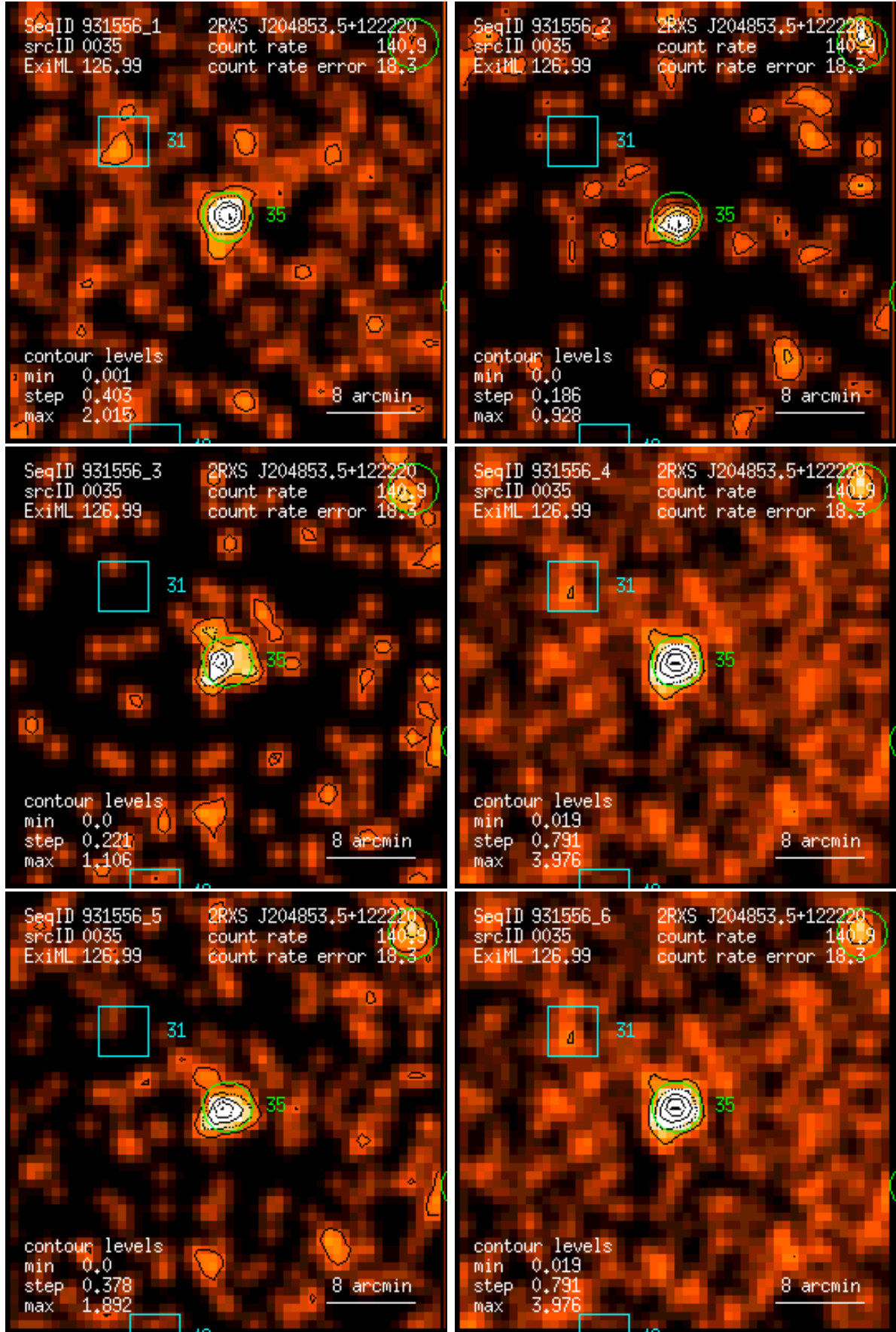
Figure 35: RASS 931556: detection 0035: band rate images, Gaussian filter: (1) PSPC channels 11 – 41, (2) 52 – 90, (3) 91 – 201, (4) 11 – 235, (5) 52 – 201, (6) 11 – 201. Broad band rates in counts/ks. Band rate contour levels in counts/ks/arcmin 2 .
