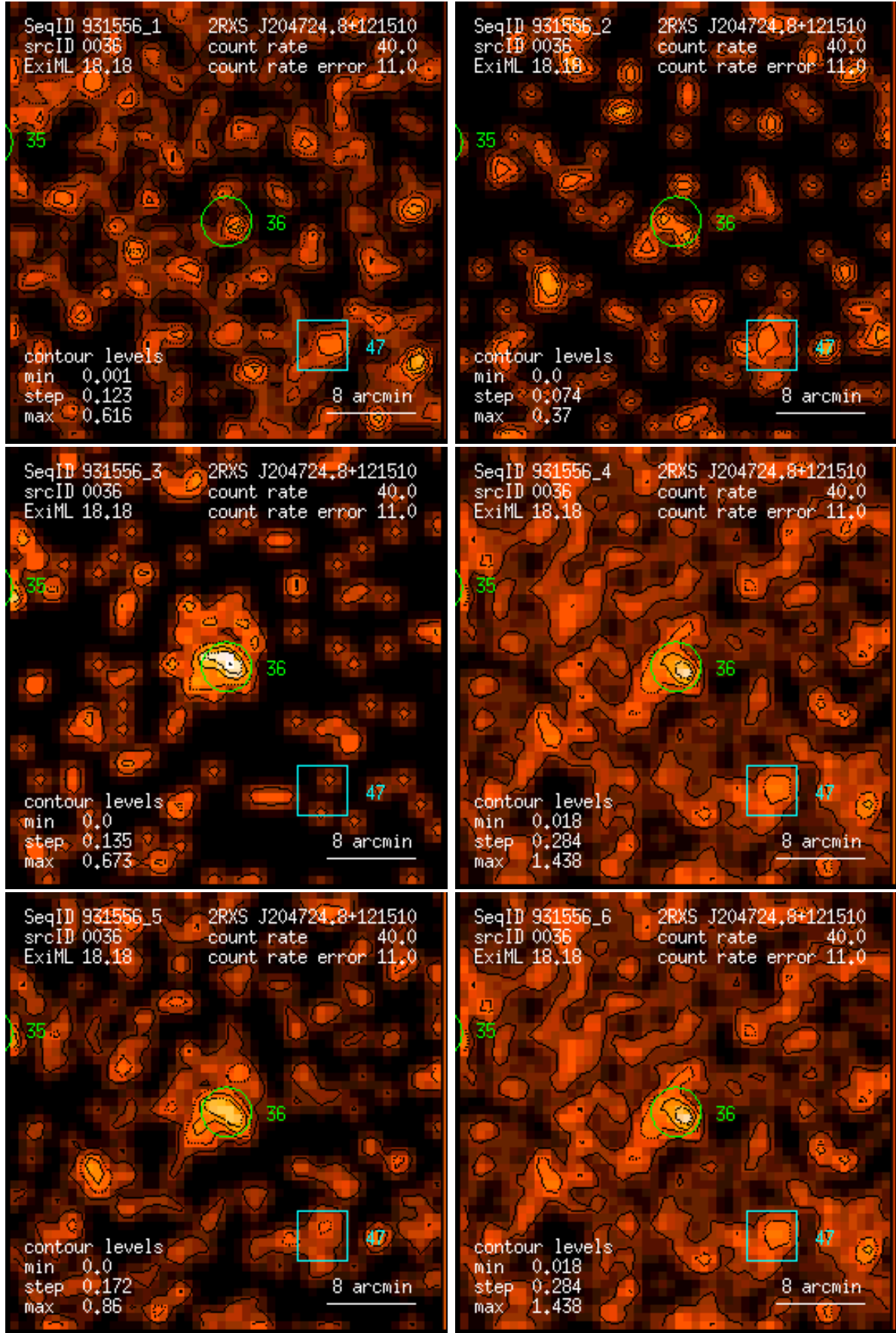
Figure 36: RASS 931556: detection 0036: band rate images, Gaussian filter: (1) PSPC channels 11 – 41, (2) 52 – 90, (3) 91 – 201, (4) 11 – 235, (5) 52 – 201, (6) 11 – 201. Broad band rates in counts/ks. Band rate contour levels in counts/ks/arcmin 2 .
