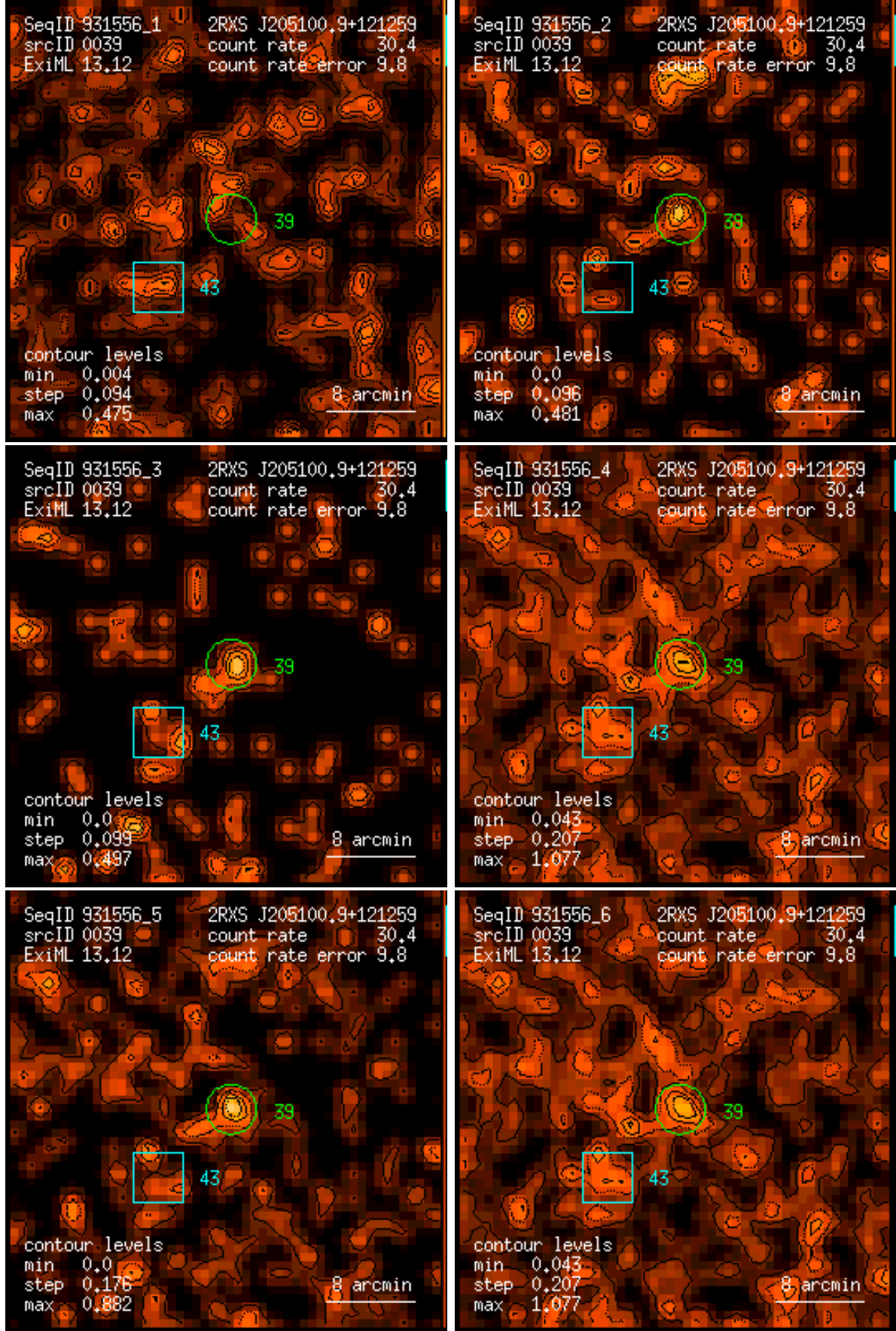
Figure 39: RASS 931556: detection 0039: band rate images, Gaussian filter: (1) PSPC channels 11 – 41, (2) 52 – 90, (3) 91 – 201, (4) 11 – 235, (5) 52 – 201, (6) 11 – 201. Broad band rates in counts/ks. Band rate contour levels in counts/ks/arcmin 2 .
