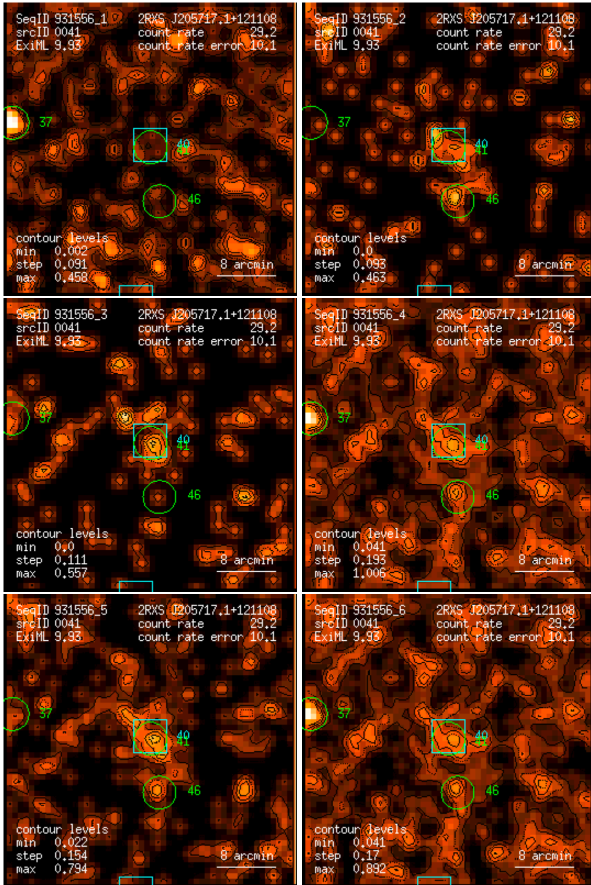
Figure 41: RASS 931556: detection 0041: band rate images, Gaussian filter: (1) PSPC channels 11 – 41, (2) 52 – 90, (3) 91 – 201, (4) 11 – 235, (5) 52 – 201, (6) 11 – 201. Broad band rates in counts/ks. Band rate contour levels in counts/ks/arcmin 2 .
