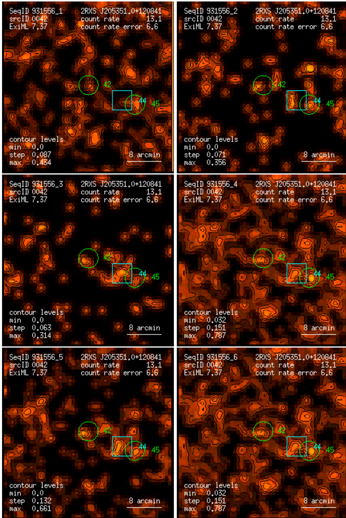
Figure 42: RASS 931556: detection 0042: band rate images, Gaussian filter: (1) PSPC channels 11 – 41, (2) 52 – 90, (3) 91 – 201, (4) 11 – 235, (5) 52 – 201, (6) 11 – 201. Broad band rates in counts/ks. Band rate contour levels in counts/ks/arcmin 2 .
