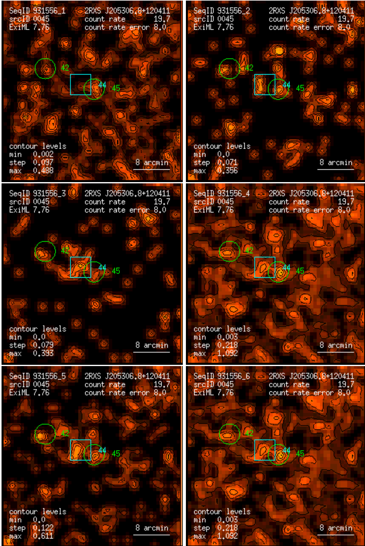
Figure 45: RASS 931556: detection 0045: band rate images, Gaussian filter: (1) PSPC channels 11 – 41, (2) 52 – 90, (3) 91 – 201, (4) 11 – 235, (5) 52 – 201, (6) 11 – 201. Broad band rates in counts/ks. Band rate contour levels in counts/ks/arcmin 2 .
