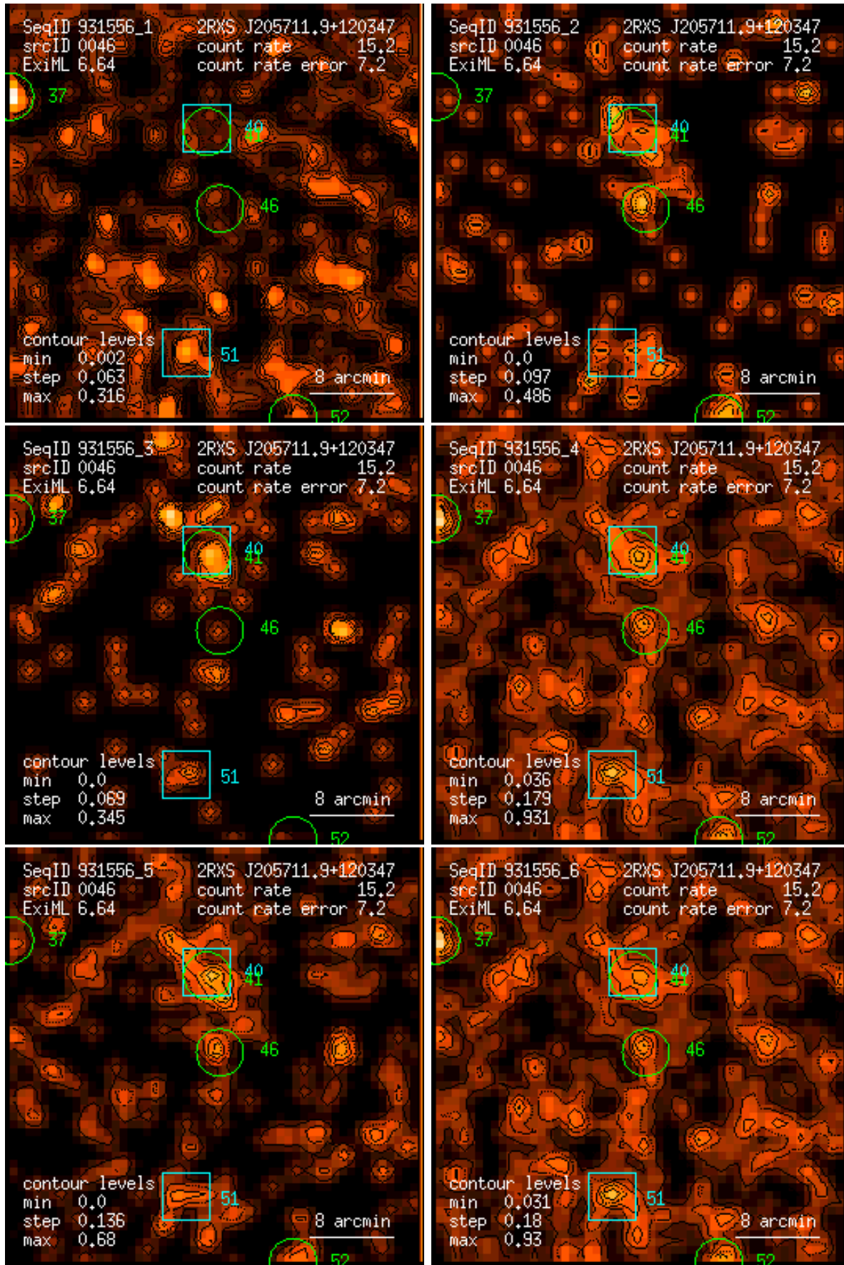
Figure 46: RASS 931556: detection 0046: band rate images, Gaussian filter: (1) PSPC channels 11 – 41, (2) 52 – 90, (3) 91 – 201, (4) 11 – 235, (5) 52 – 201, (6) 11 – 201. Broad band rates in counts/ks. Band rate contour levels in counts/ks/arcmin 2 .
