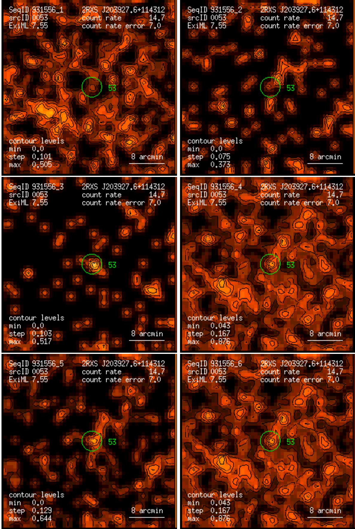
Figure 53: RASS 931556: detection 0053: band rate images, Gaussian filter: (1) PSPC channels 11 – 41, (2) 52 – 90, (3) 91 – 201, (4) 11 – 235, (5) 52 – 201, (6) 11 – 201. Broad band rates in counts/ks. Band rate contour levels in counts/ks/arcmin 2 .
