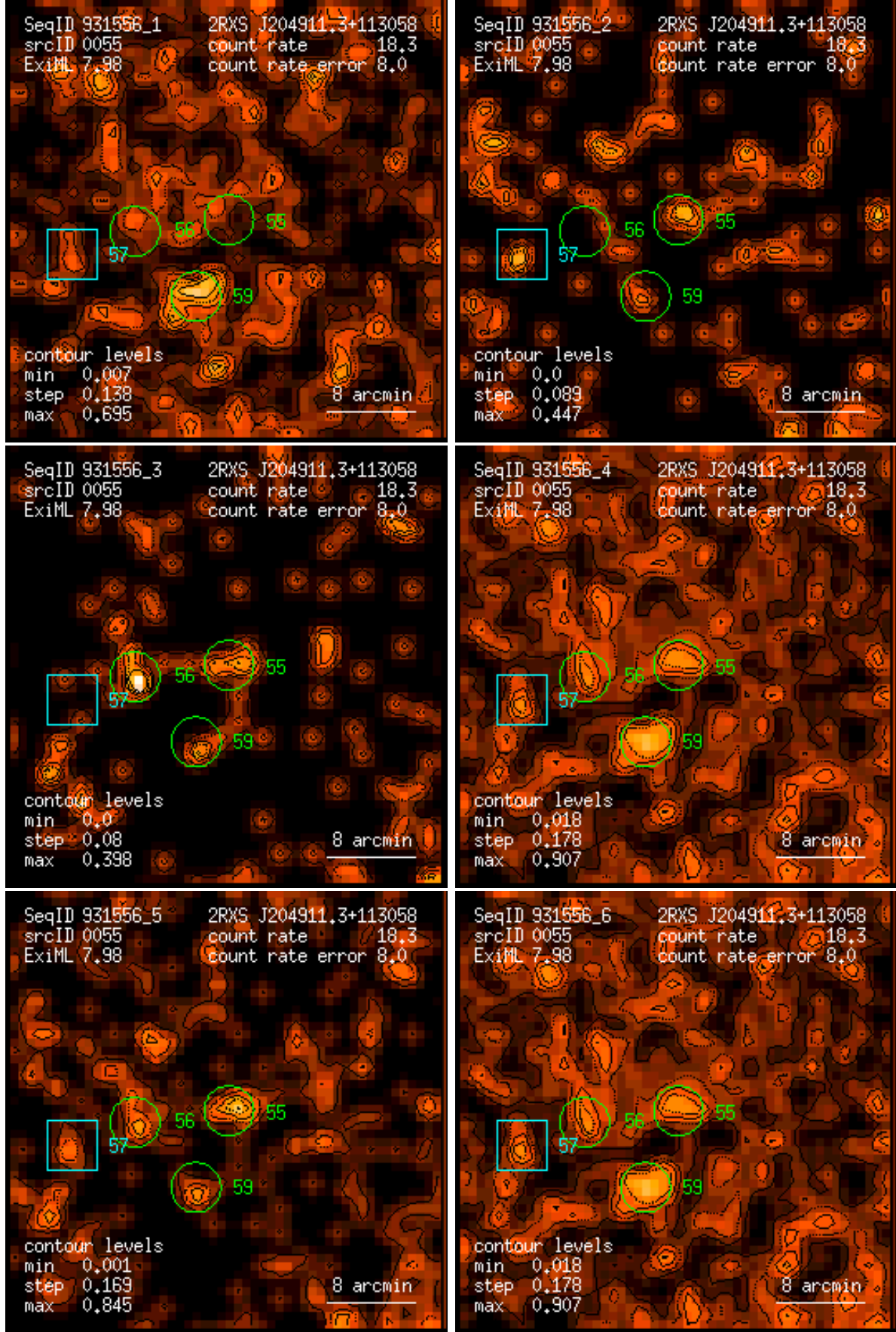
Figure 55: RASS 931556: detection 0055: band rate images, Gaussian filter: (1) PSPC channels 11 – 41, (2) 52 – 90, (3) 91 – 201, (4) 11 – 235, (5) 52 – 201, (6) 11 – 201. Broad band rates in counts/ks. Band rate contour levels in counts/ks/arcmin 2 .
