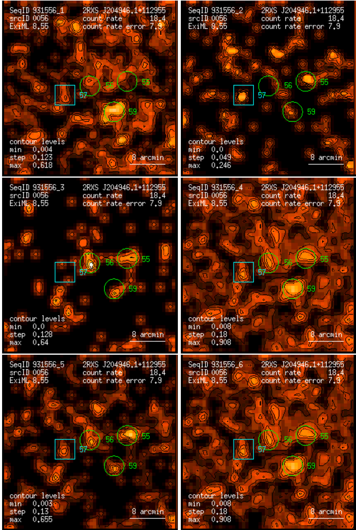
Figure 56: RASS 931556: detection 0056: band rate images, Gaussian filter: (1) PSPC channels 11 – 41, (2) 52 – 90, (3) 91 – 201, (4) 11 – 235, (5) 52 – 201, (6) 11 – 201. Broad band rates in counts/ks. Band rate contour levels in counts/ks/arcmin 2 .
