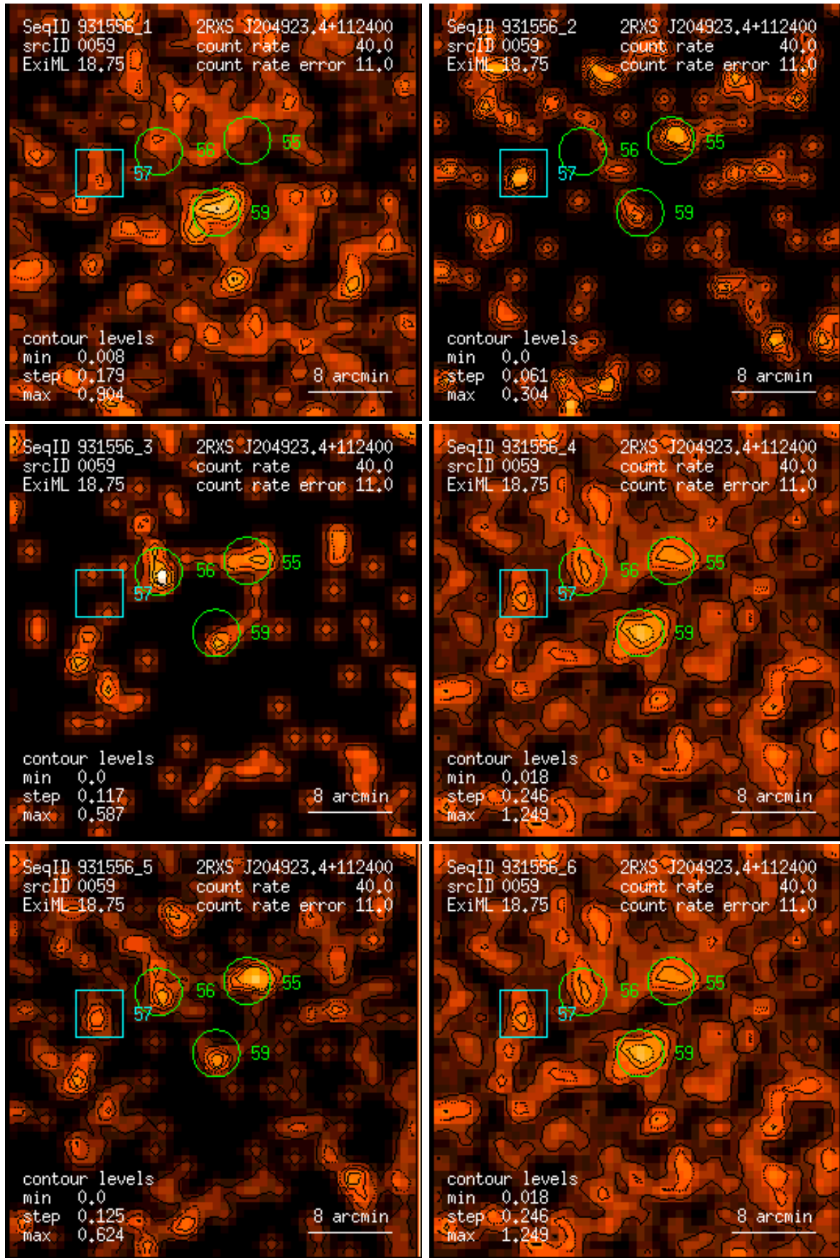
Figure 59: RASS 931556: detection 0059: band rate images, Gaussian filter: (1) PSPC channels 11 – 41, (2) 52 – 90, (3) 91 – 201, (4) 11 – 235, (5) 52 – 201, (6) 11 – 201. Broad band rates in counts/ks. Band rate contour levels in counts/ks/arcmin 2 .
