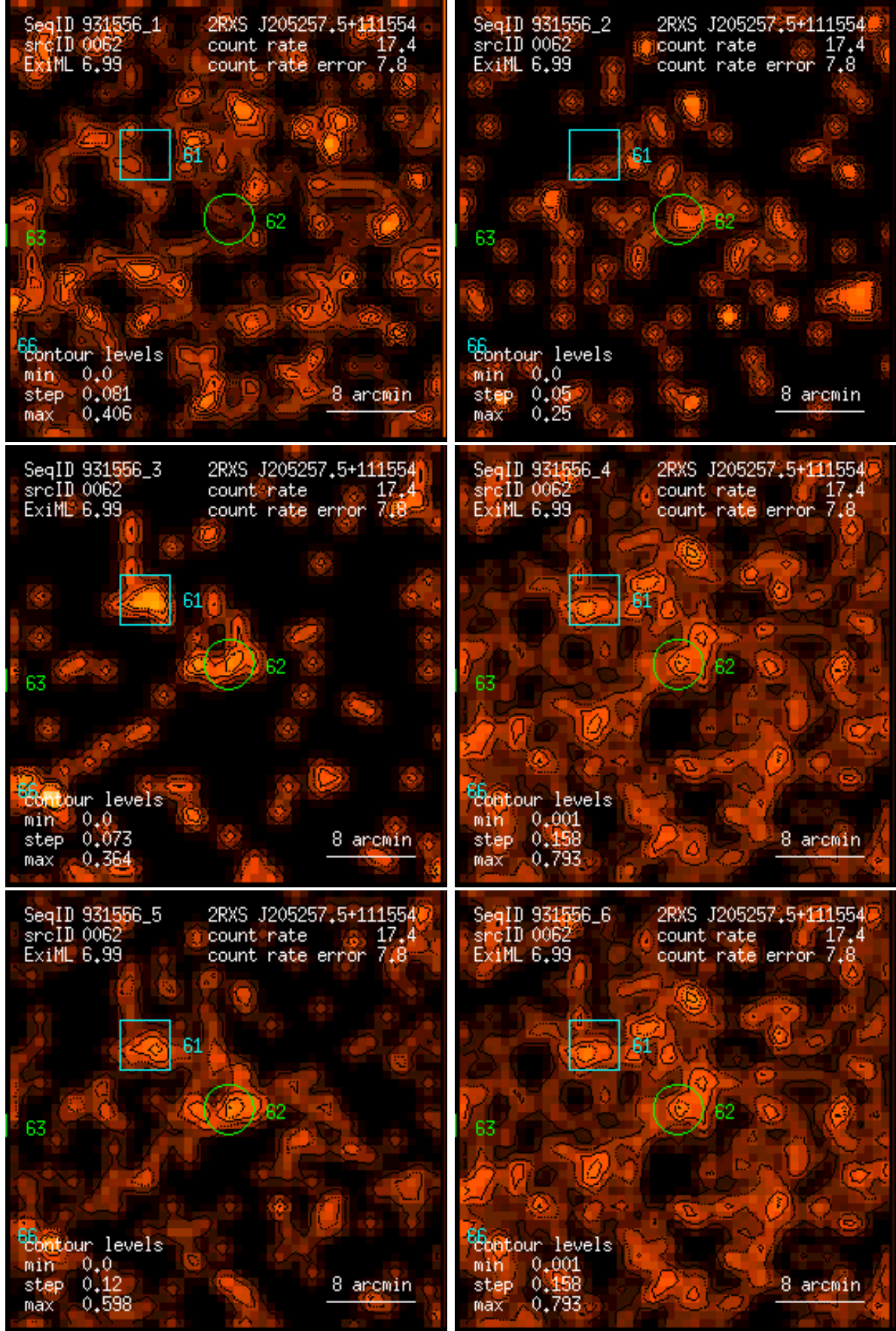
Figure 62: RASS 931556: detection 0062: band rate images, Gaussian filter: (1) PSPC channels 11 – 41, (2) 52 – 90, (3) 91 – 201, (4) 11 – 235, (5) 52 – 201, (6) 11 – 201. Broad band rates in counts/ks. Band rate contour levels in counts/ks/arcmin 2 .
