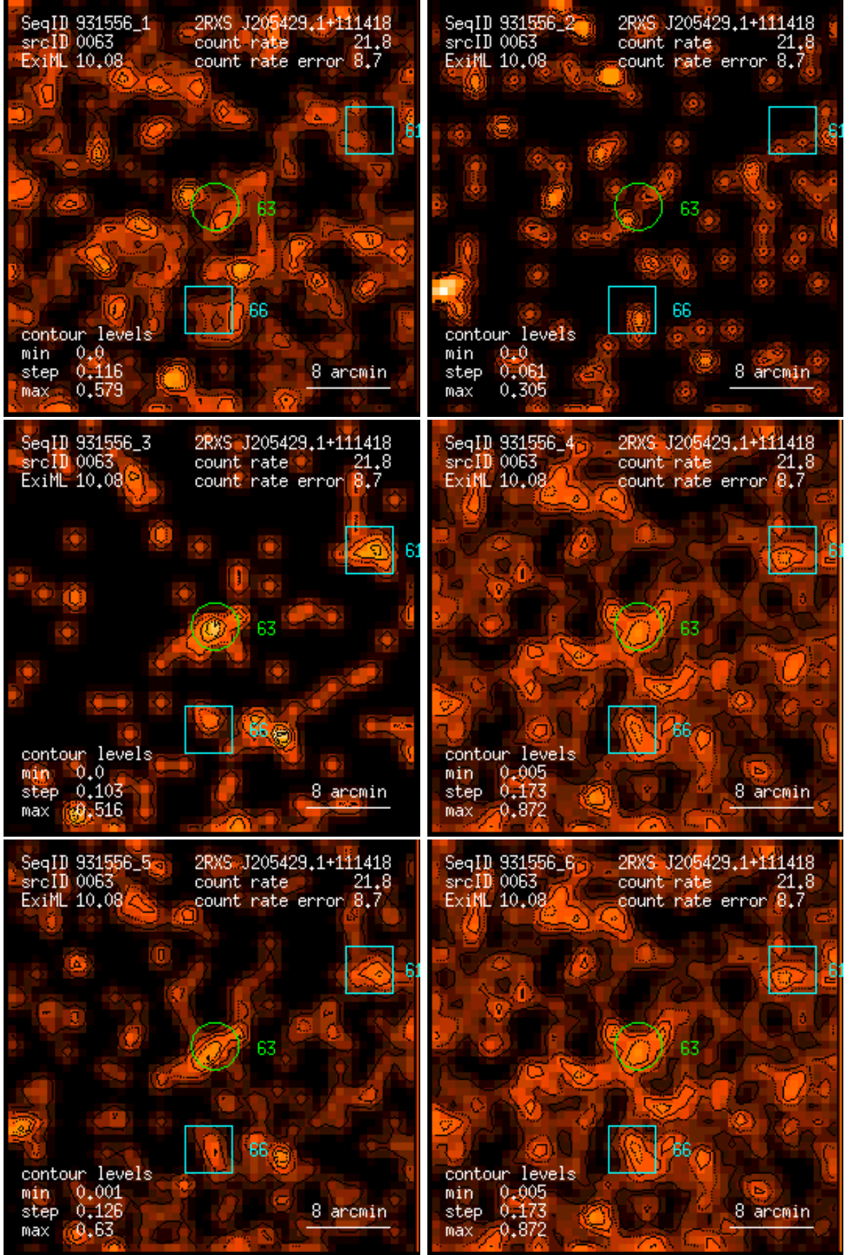
Figure 63: RASS 931556: detection 0063: band rate images, Gaussian filter: (1) PSPC channels 11 – 41, (2) 52 – 90, (3) 91 – 201, (4) 11 – 235, (5) 52 – 201, (6) 11 – 201. Broad band rates in counts/ks. Band rate contour levels in counts/ks/arcmin 2 .
