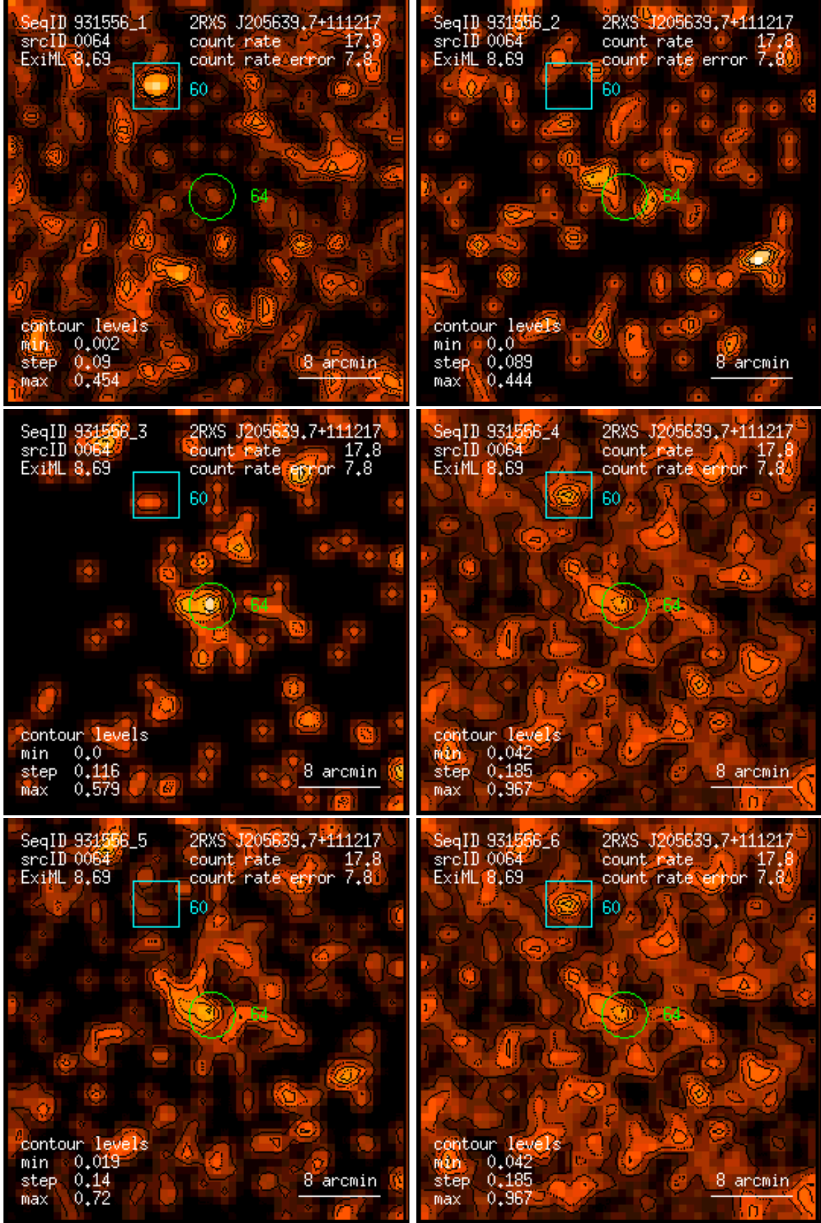
Figure 64: RASS 931556: detection 0064: band rate images, Gaussian filter: (1) PSPC channels 11 – 41, (2) 52 – 90, (3) 91 – 201, (4) 11 – 235, (5) 52 – 201, (6) 11 – 201. Broad band rates in counts/ks. Band rate contour levels in counts/ks/arcmin 2 .
