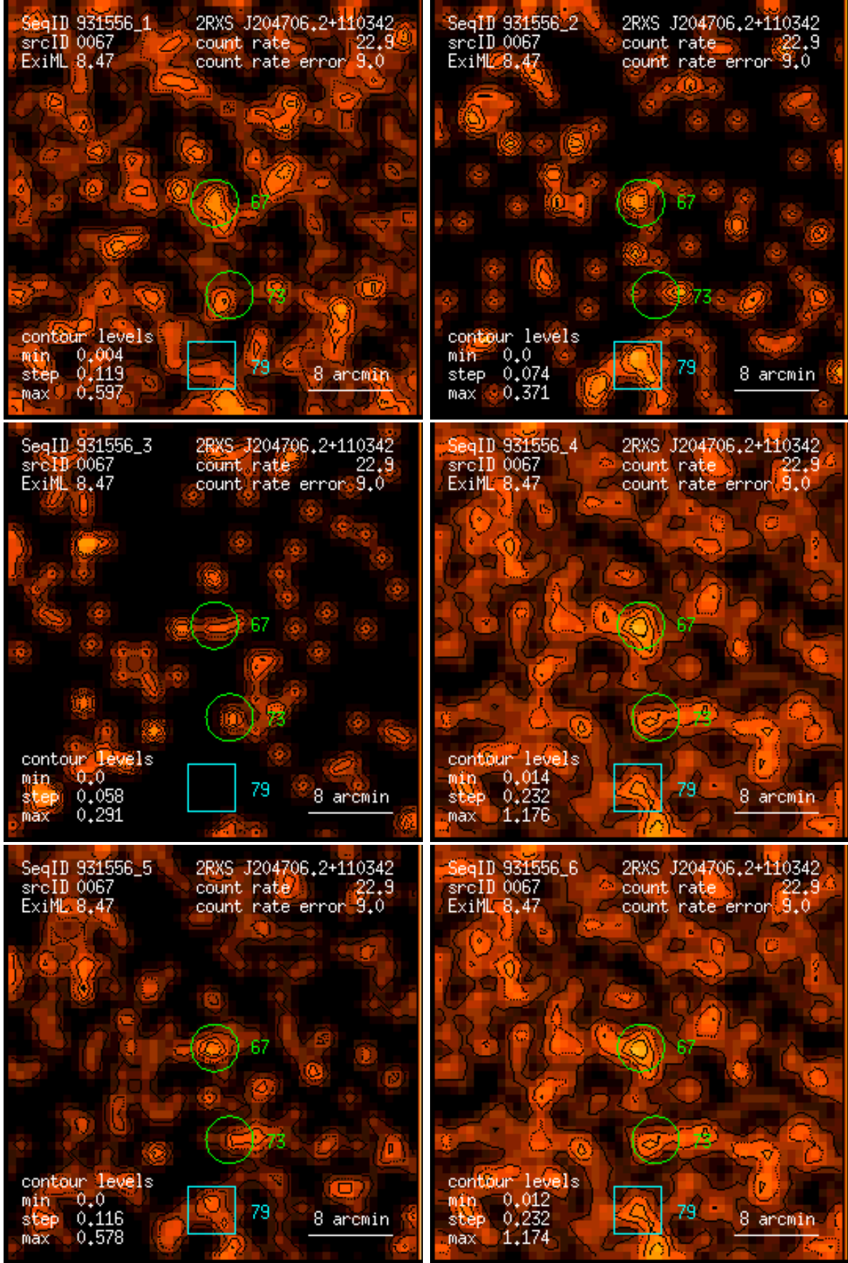
Figure 67: RASS 931556: detection 0067: band rate images, Gaussian filter: (1) PSPC channels 11 – 41, (2) 52 – 90, (3) 91 – 201, (4) 11 – 235, (5) 52 – 201, (6) 11 – 201. Broad band rates in counts/ks. Band rate contour levels in counts/ks/arcmin 2 .
