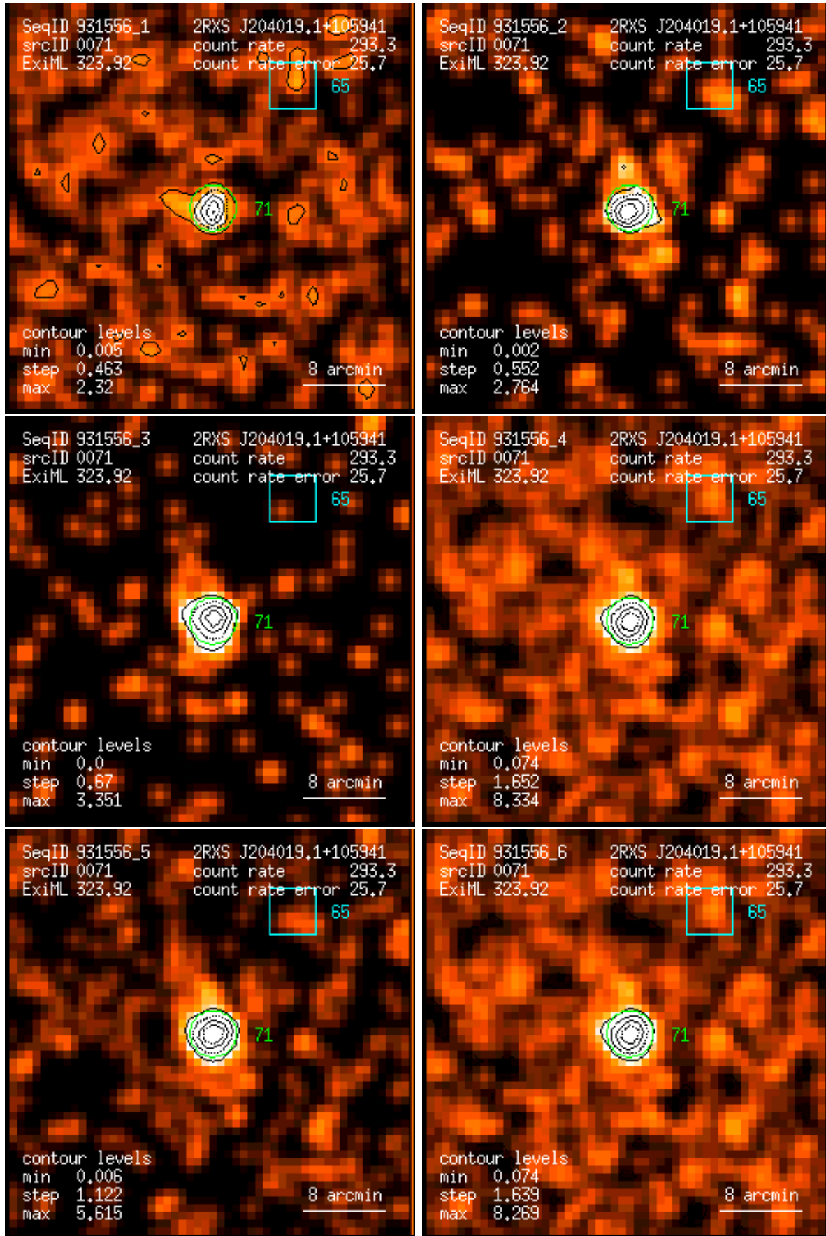
Figure 71: RASS 931556: detection 0071: band rate images, Gaussian filter: (1) PSPC channels 11 – 41, (2) 52 – 90, (3) 91 – 201, (4) 11 – 235, (5) 52 – 201, (6) 11 – 201. Broad band rates in counts/ks. Band rate contour levels in counts/ks/arcmin 2 .
