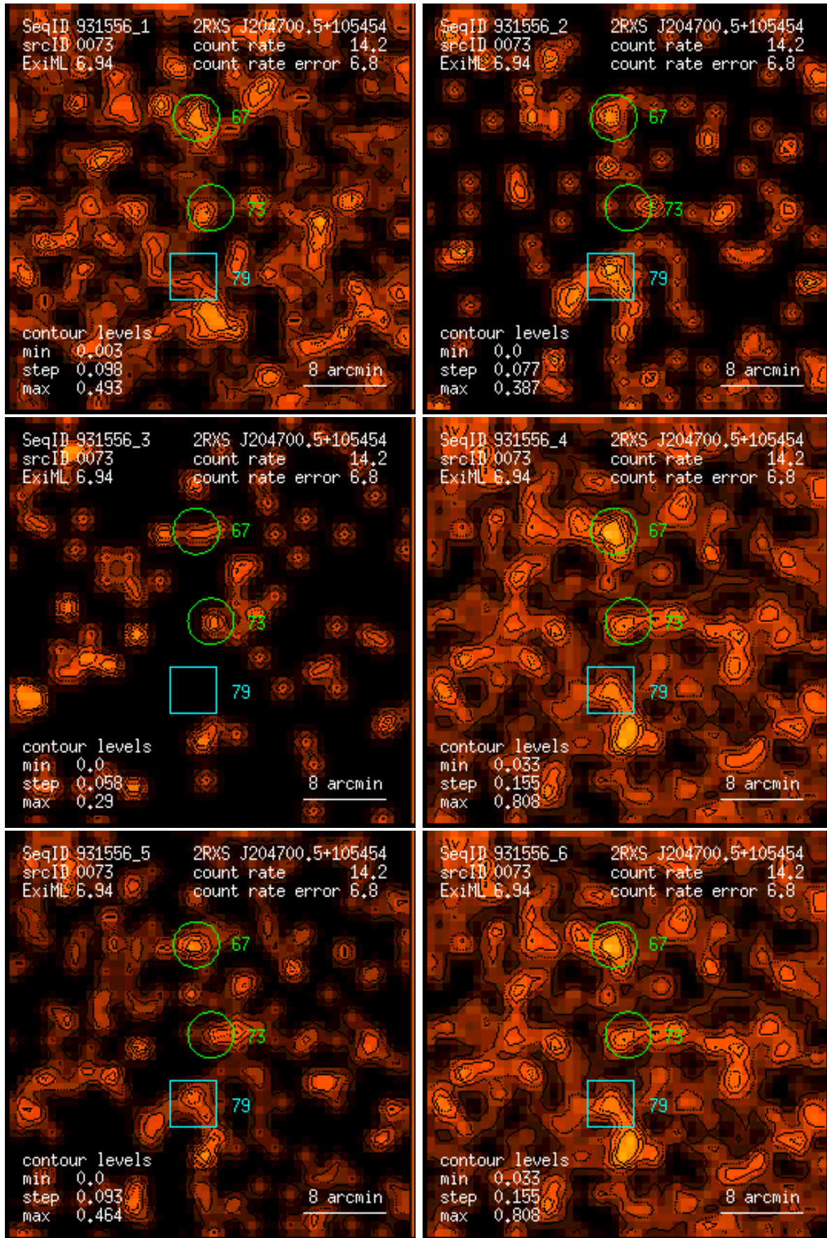
Figure 73: RASS 931556: detection 0073: band rate images, Gaussian filter: (1) PSPC channels 11 – 41, (2) 52 – 90, (3) 91 – 201, (4) 11 – 235, (5) 52 – 201, (6) 11 – 201. Broad band rates in counts/ks. Band rate contour levels in counts/ks/arcmin 2 .
