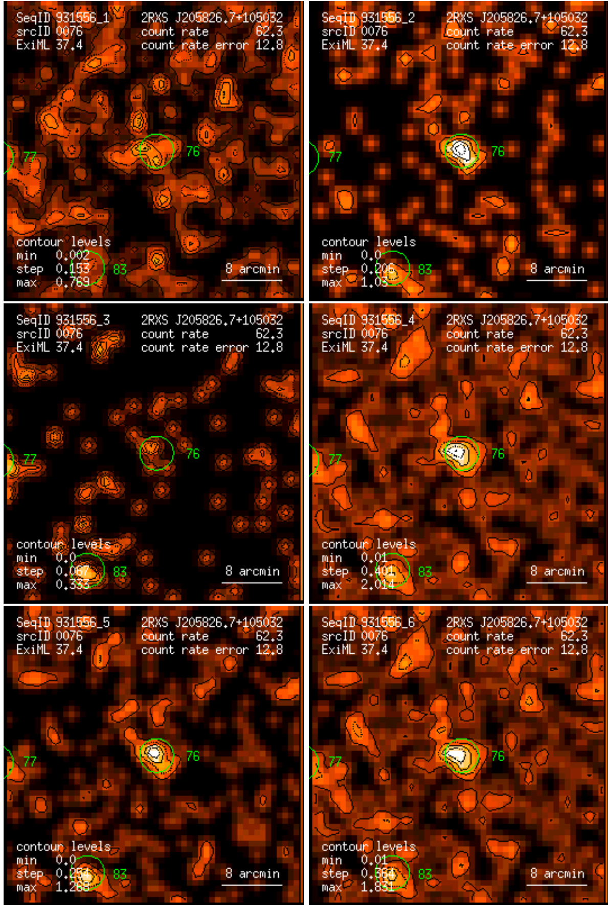
Figure 76: RASS 931556: detection 0076: band rate images, Gaussian filter: (1) PSPC channels 11 – 41, (2) 52 – 90, (3) 91 – 201, (4) 11 – 235, (5) 52 – 201, (6) 11 – 201. Broad band rates in counts/ks. Band rate contour levels in counts/ks/arcmin 2 .
