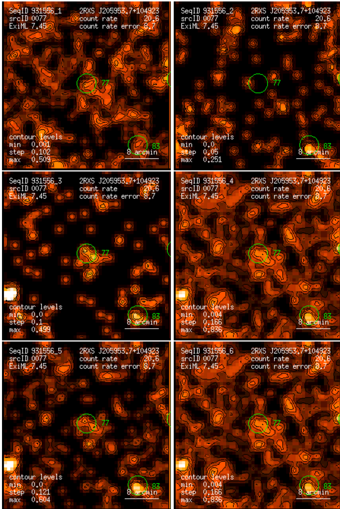
Figure 77: RASS 931556: detection 0077: band rate images, Gaussian filter: (1) PSPC channels 11 – 41, (2) 52 – 90, (3) 91 – 201, (4) 11 – 235, (5) 52 – 201, (6) 11 – 201. Broad band rates in counts/ks. Band rate contour levels in counts/ks/arcmin 2 .
