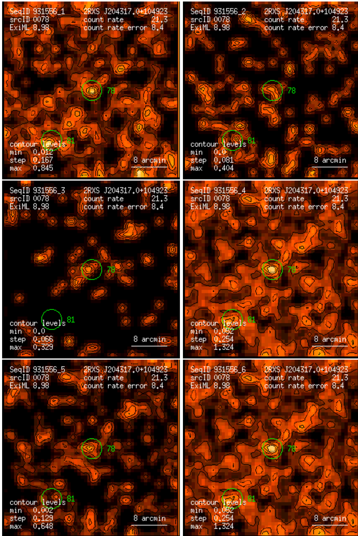
Figure 78: RASS 931556: detection 0078: band rate images, Gaussian filter: (1) PSPC channels 11 – 41, (2) 52 – 90, (3) 91 – 201, (4) 11 – 235, (5) 52 – 201, (6) 11 – 201. Broad band rates in counts/ks. Band rate contour levels in counts/ks/arcmin 2 .
