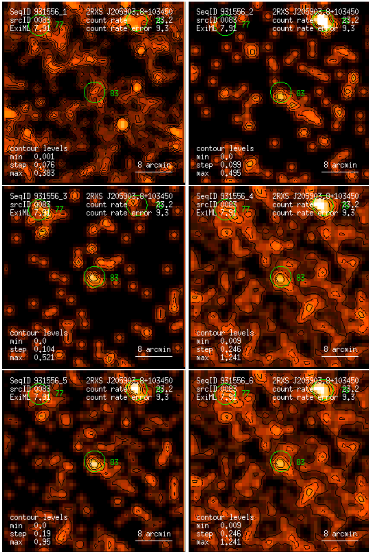
Figure 83: RASS 931556: detection 0083: band rate images, Gaussian filter: (1) PSPC channels 11 – 41, (2) 52 – 90, (3) 91 – 201, (4) 11 – 235, (5) 52 – 201, (6) 11 – 201. Broad band rates in counts/ks. Band rate contour levels in counts/ks/arcmin 2 .
