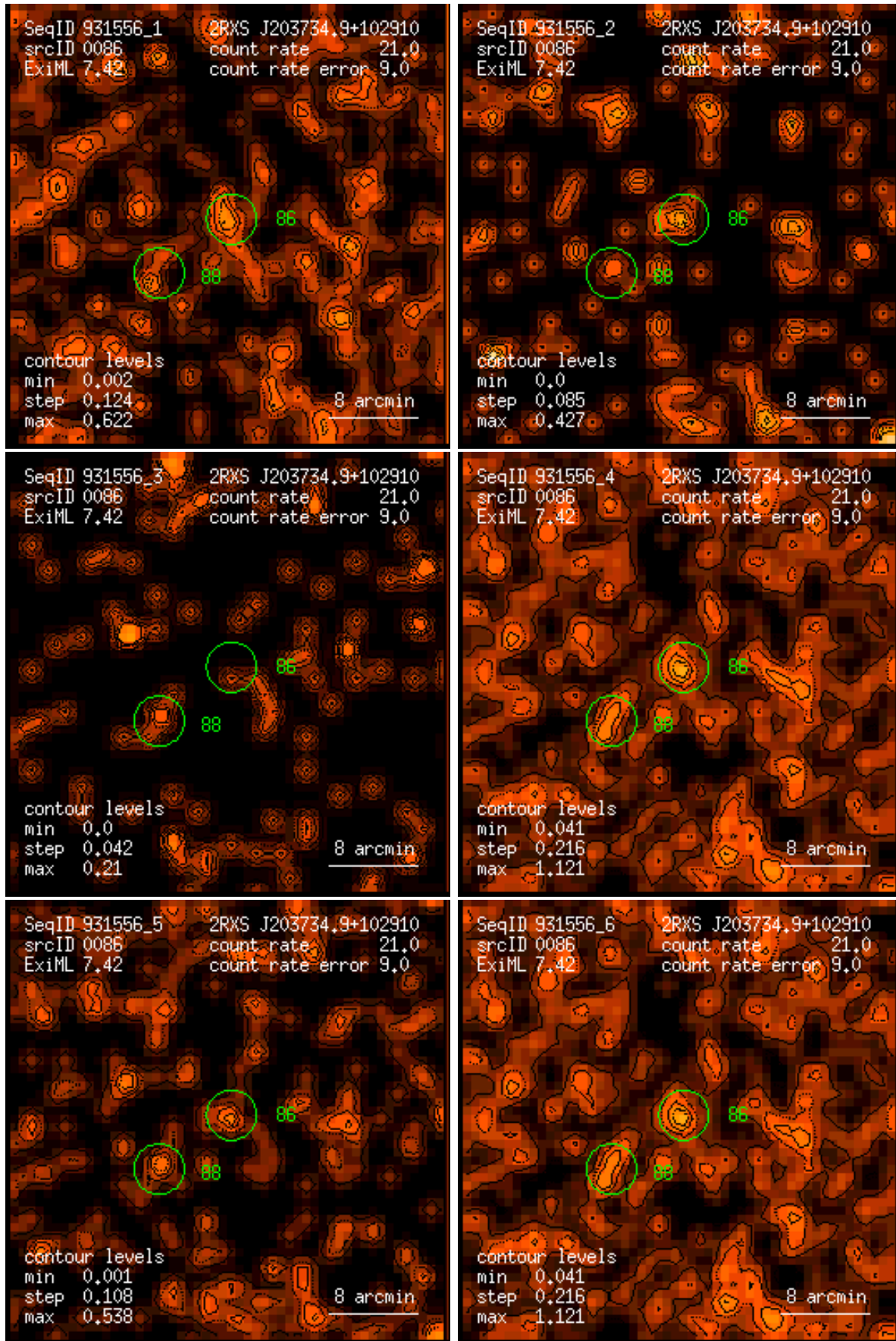
Figure 86: RASS 931556: detection 0086: band rate images, Gaussian filter: (1) PSPC channels 11 – 41, (2) 52 – 90, (3) 91 – 201, (4) 11 – 235, (5) 52 – 201, (6) 11 – 201. Broad band rates in counts/ks. Band rate contour levels in counts/ks/arcmin 2 .
